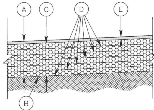
STRUCTURAL SECTION DETAIL NTS
