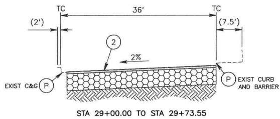
TYPICAL SECTIONS - GLEN HELEN PARKWAY NTS
