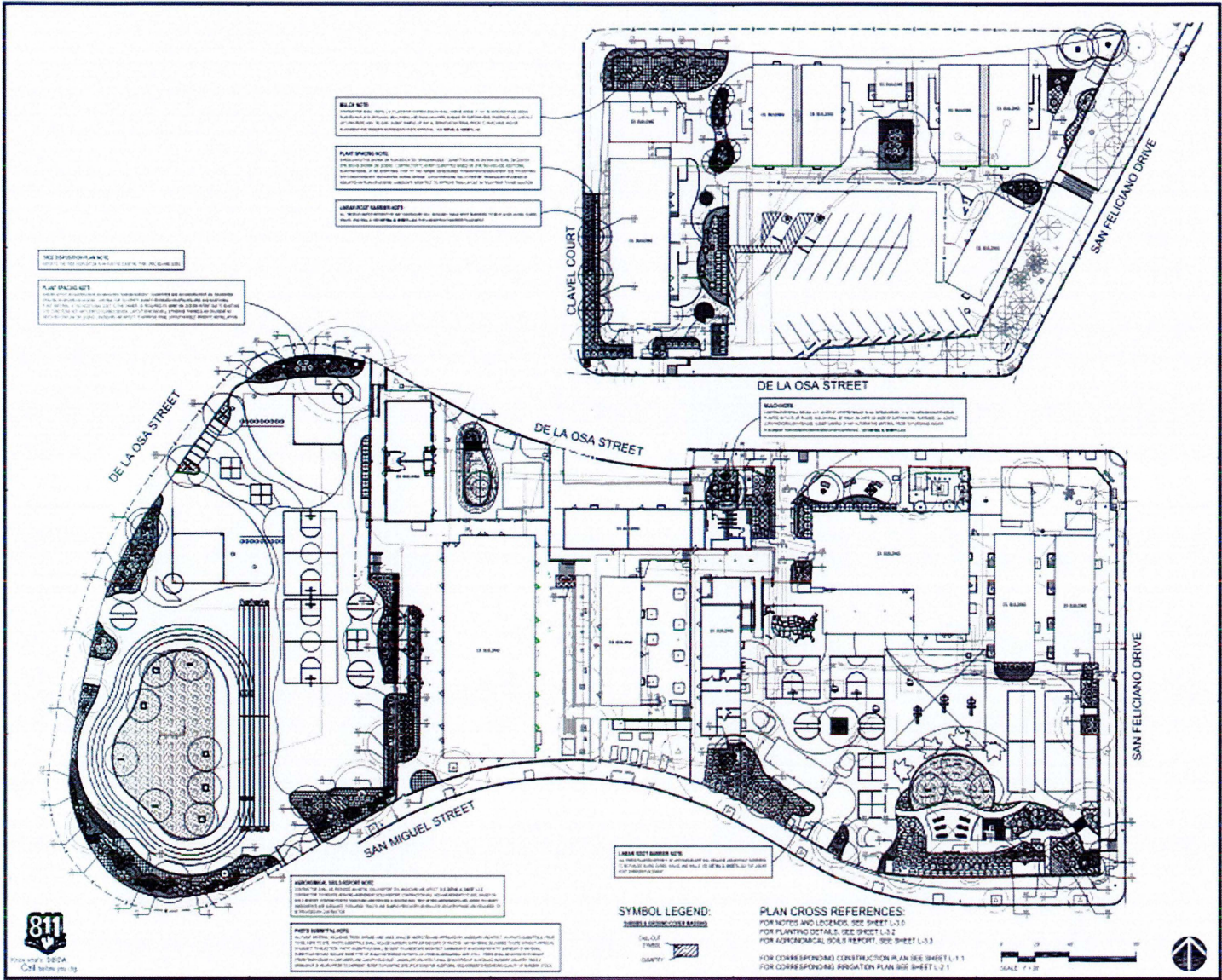
Figure 1. Project Site Plan
