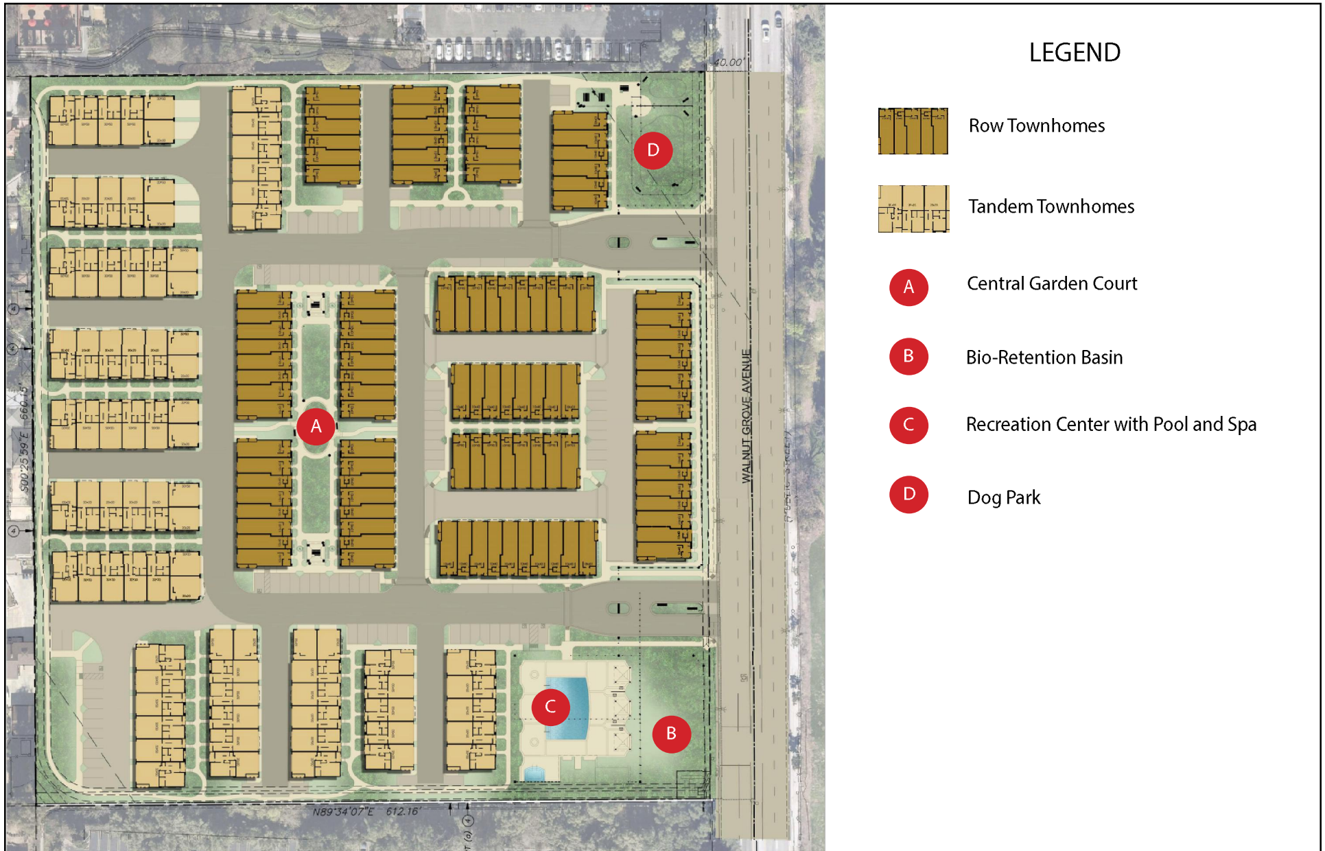
FIGURE 2.4-1: Site Plan
