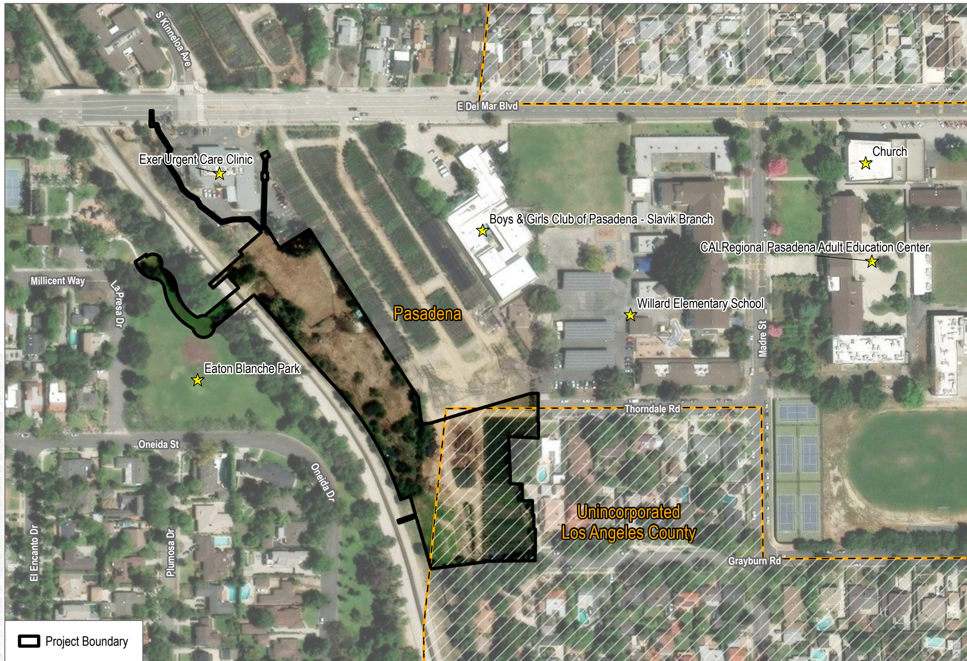
FIGURE 2 Project Site Eaton Wash Stormwater Capture Project
