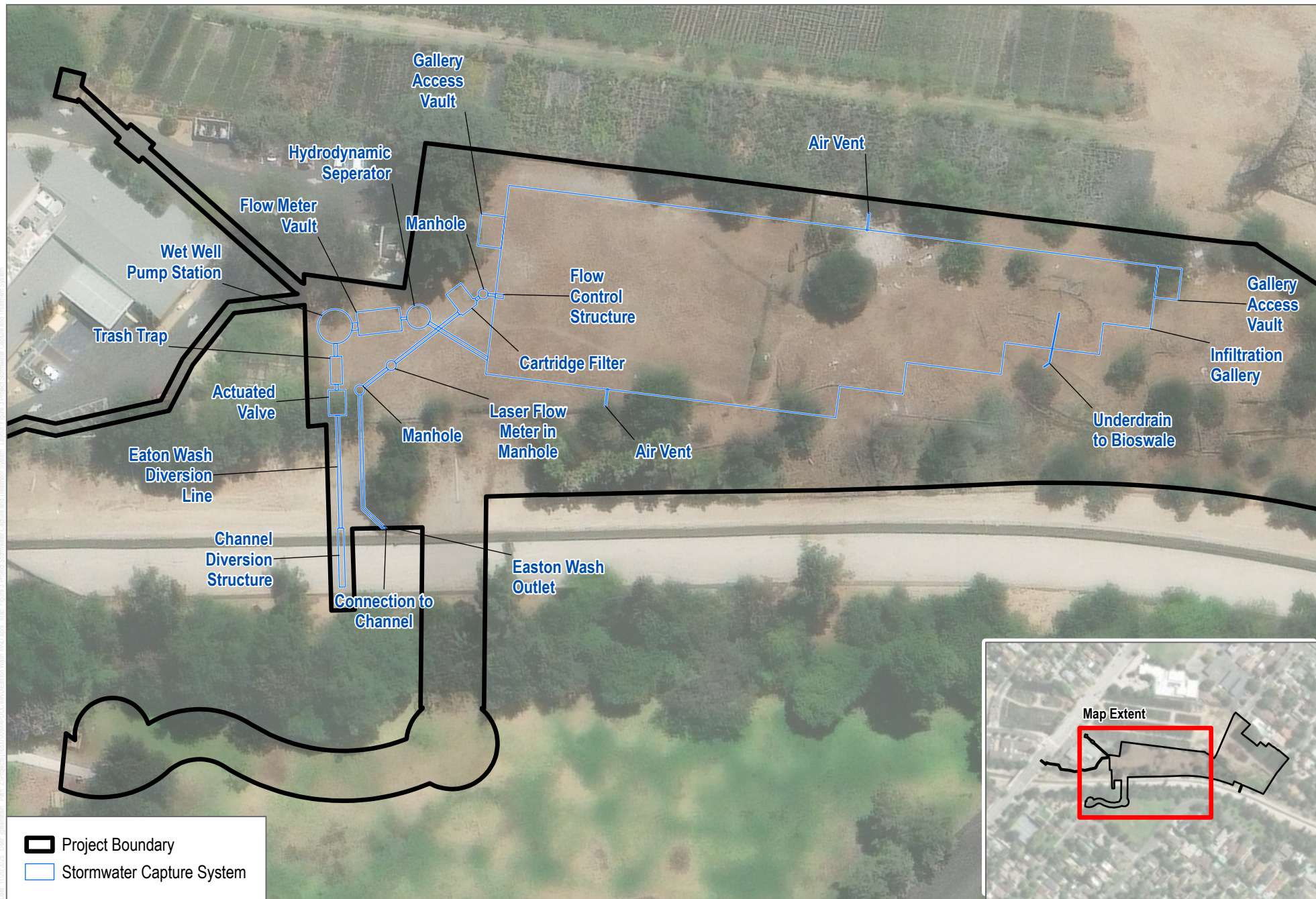
FIGURE 3 Project Stormwater Capture and Treatment System
