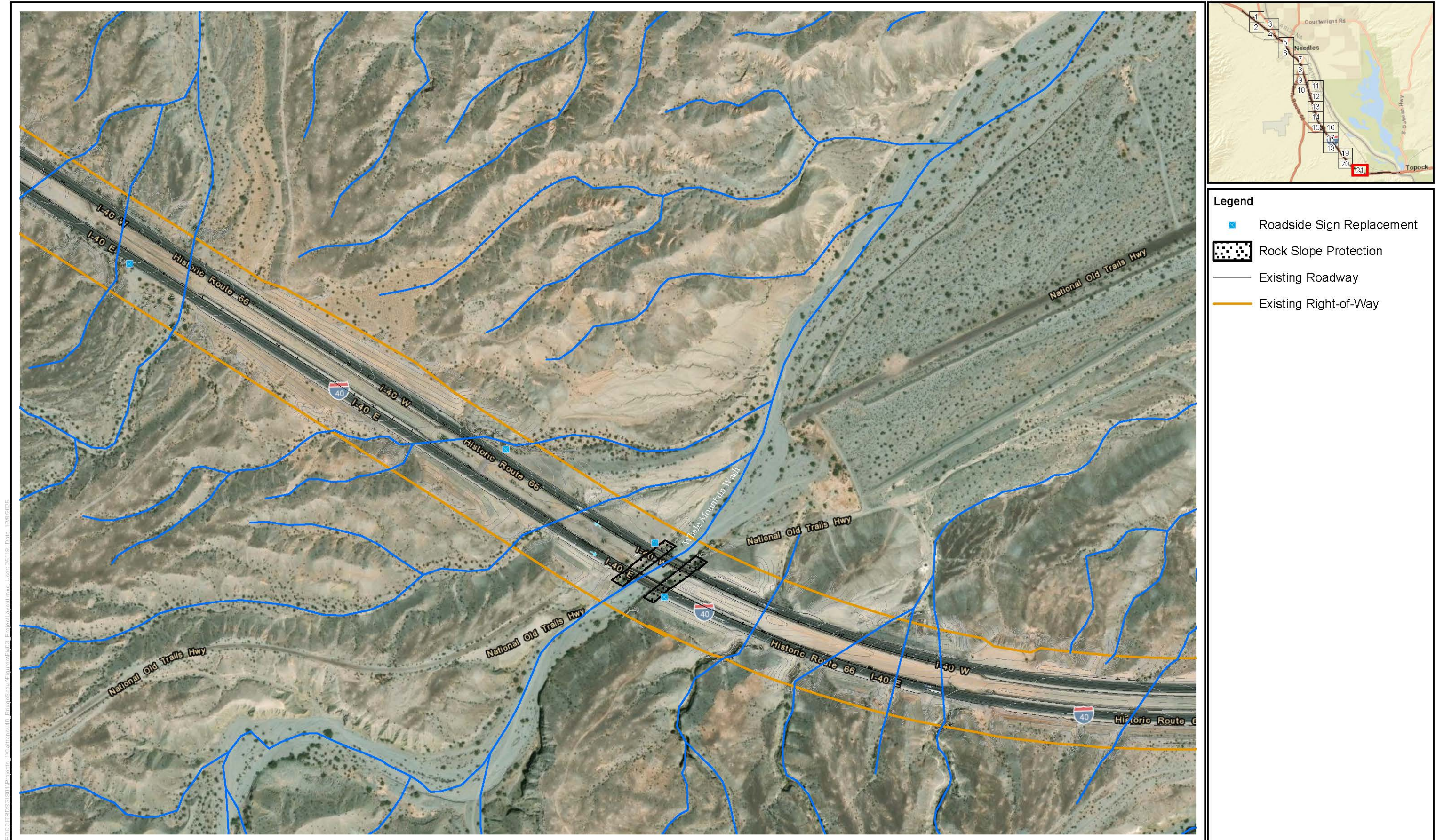
Figure 3 - Sheet 21 of 21 Project Layout I-40 Bridge Scour Project
