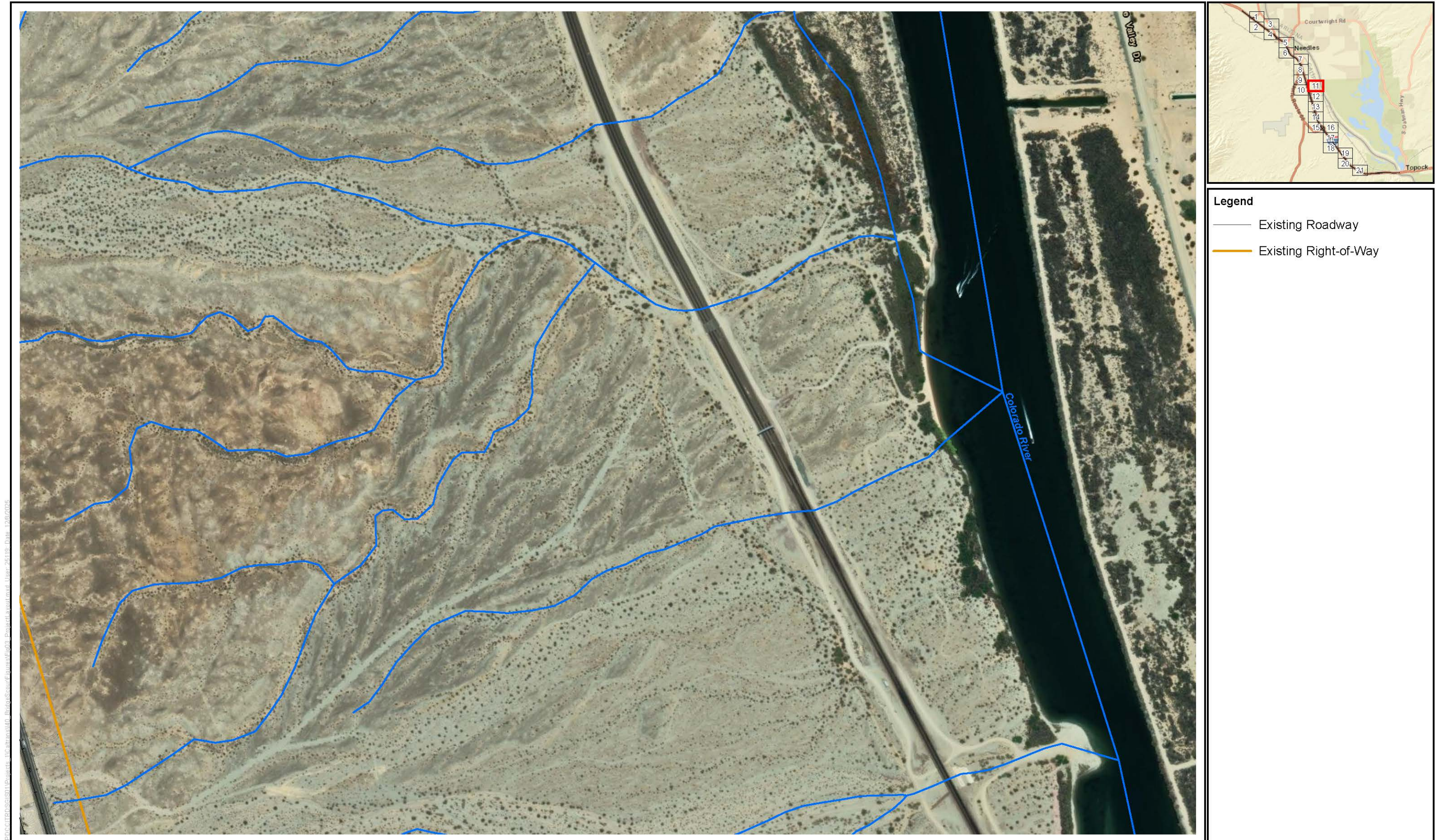
Figure 3 - Sheet 11 of 21 Project Layout I-40 Bridge Scour Project
