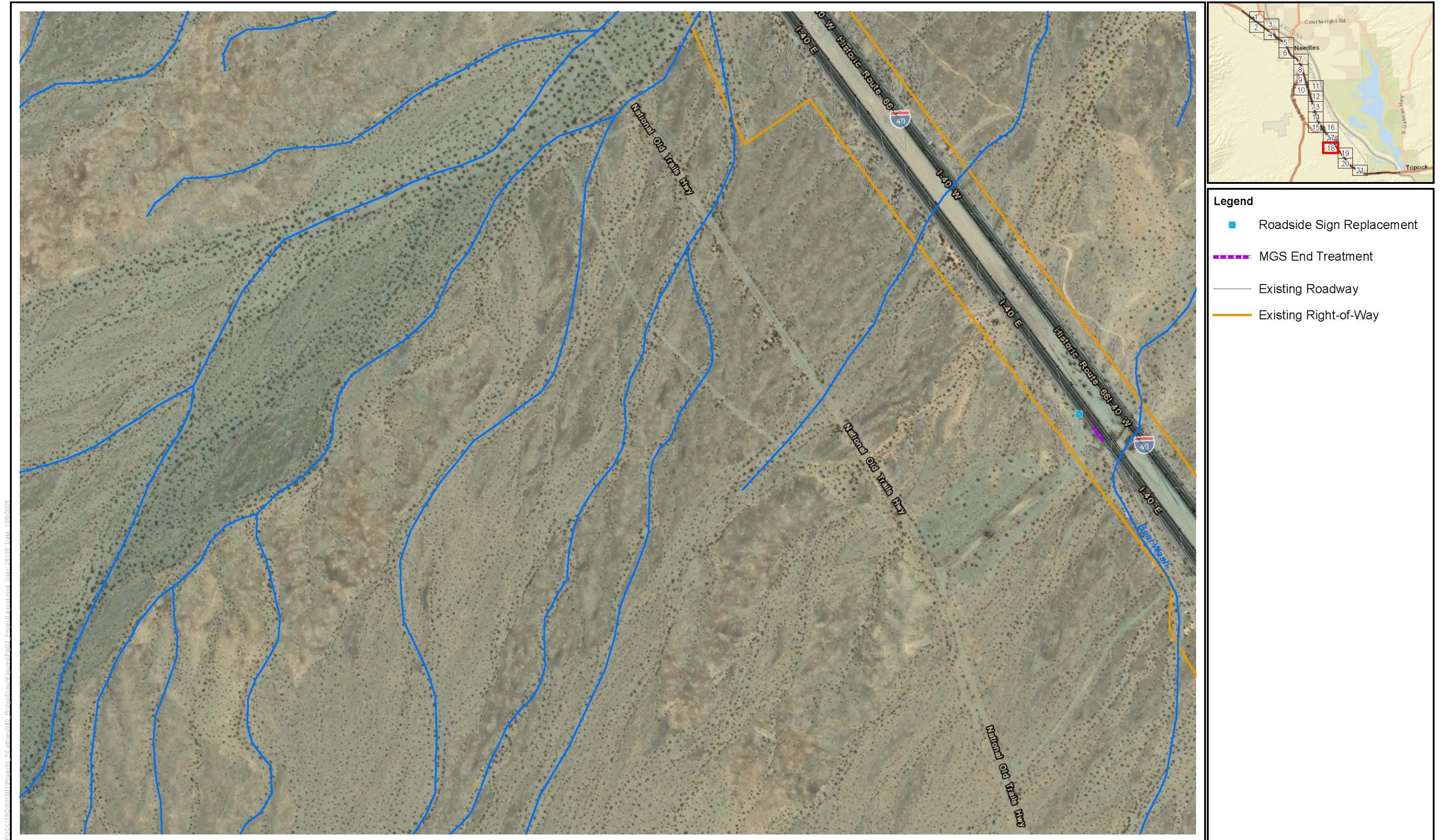
Figure 3 - Sheet 18 of 21 Project Layout I-40 Bridge Scour Project
