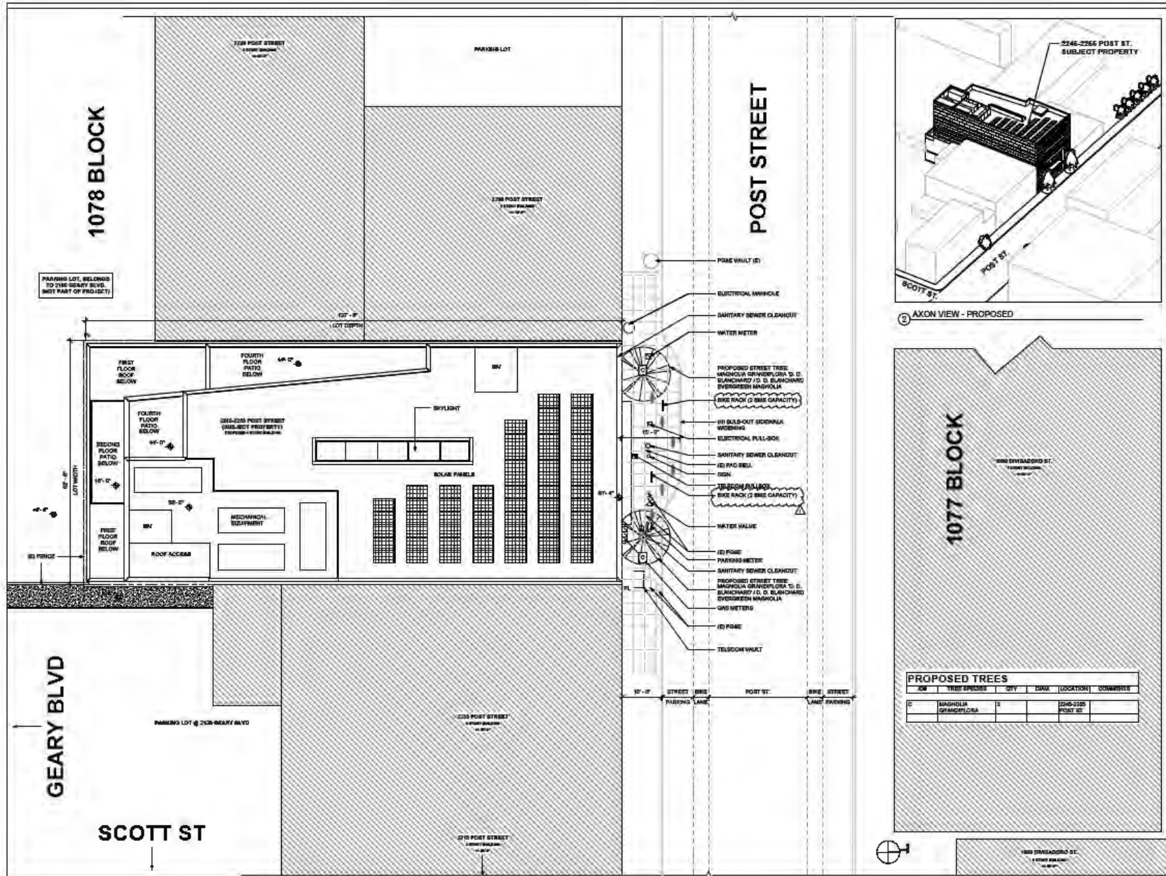
FIGURE 2 SITE PLAN
