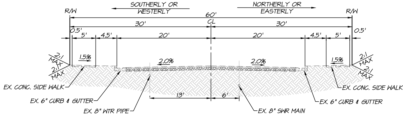
TYPICAL TTM 38605 STREET SECTION (PUBLIC)
