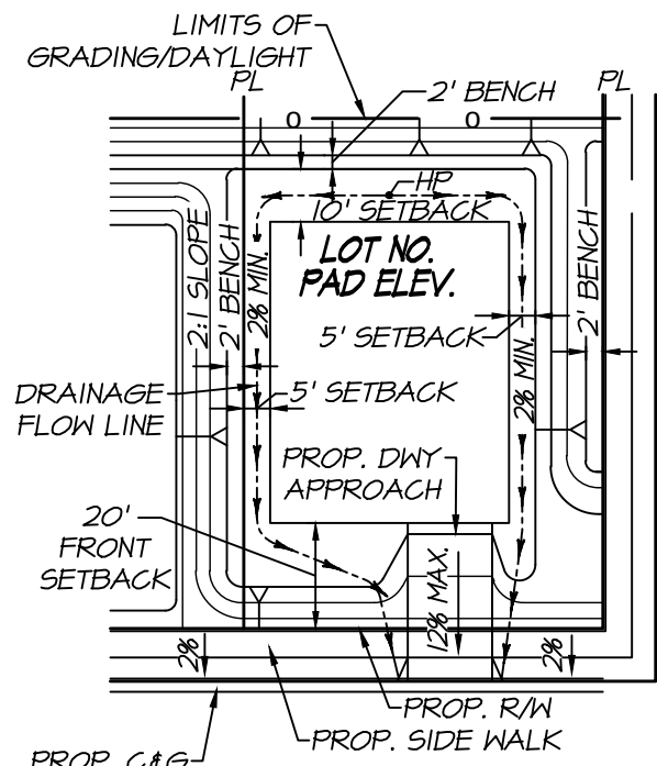
TYPICAL PAD & LOT DATA
