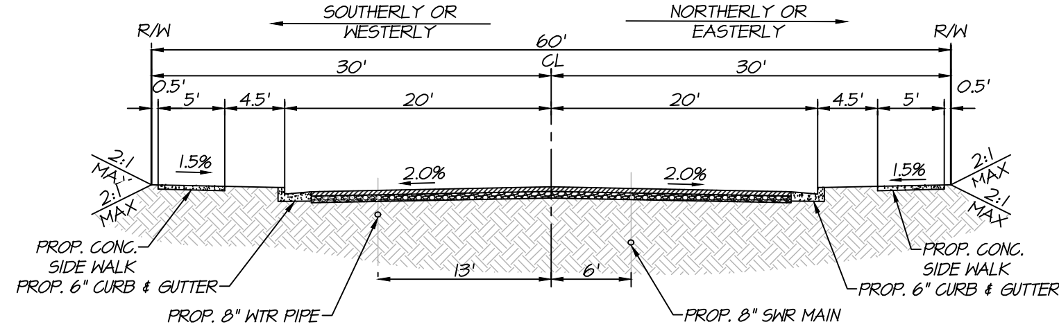
TYPICAL PUBLIC STREET SECTION OFFSITE STREET "G" SCALE: 1" = 10'
