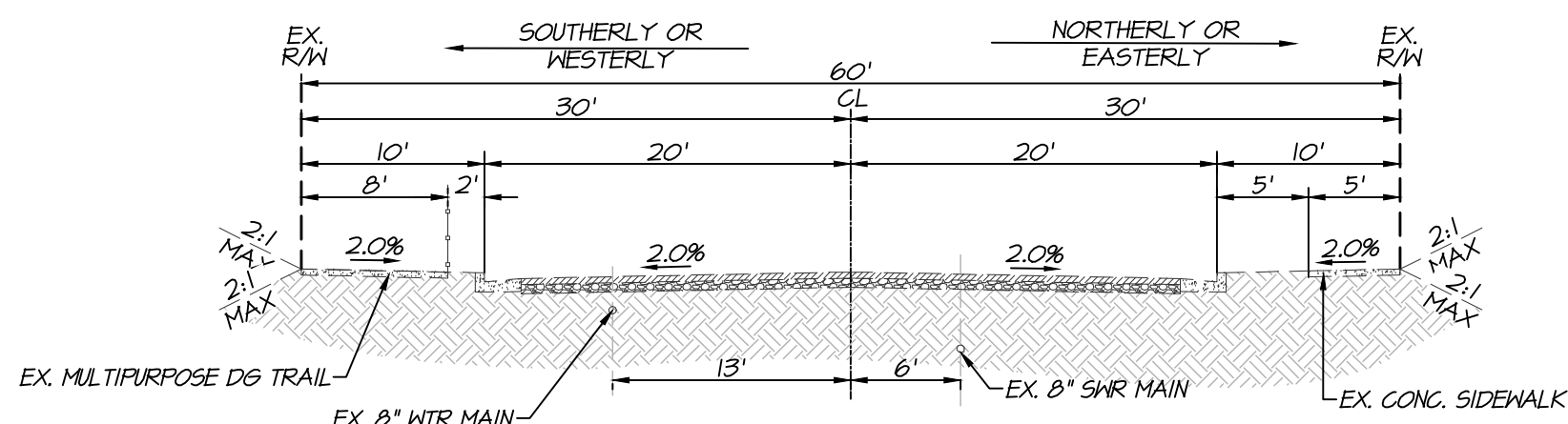
EX. TYPICAL TRAVERTINE DR. SECTION SCALE: 1" = 10'
