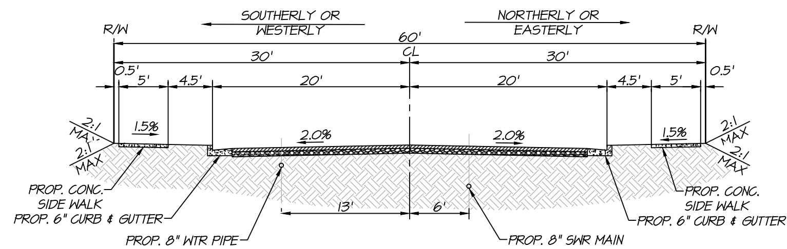
TYPICAL PUBLIC STREET SECTION STREET "A" - "G" SCALE: 1" = 10'
