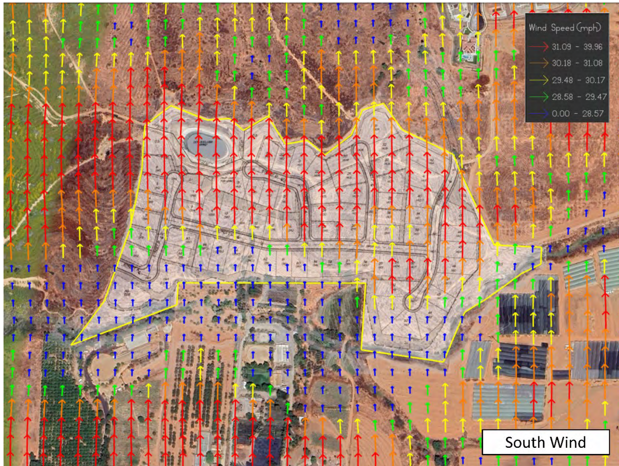
Figure 21 – South Wind
