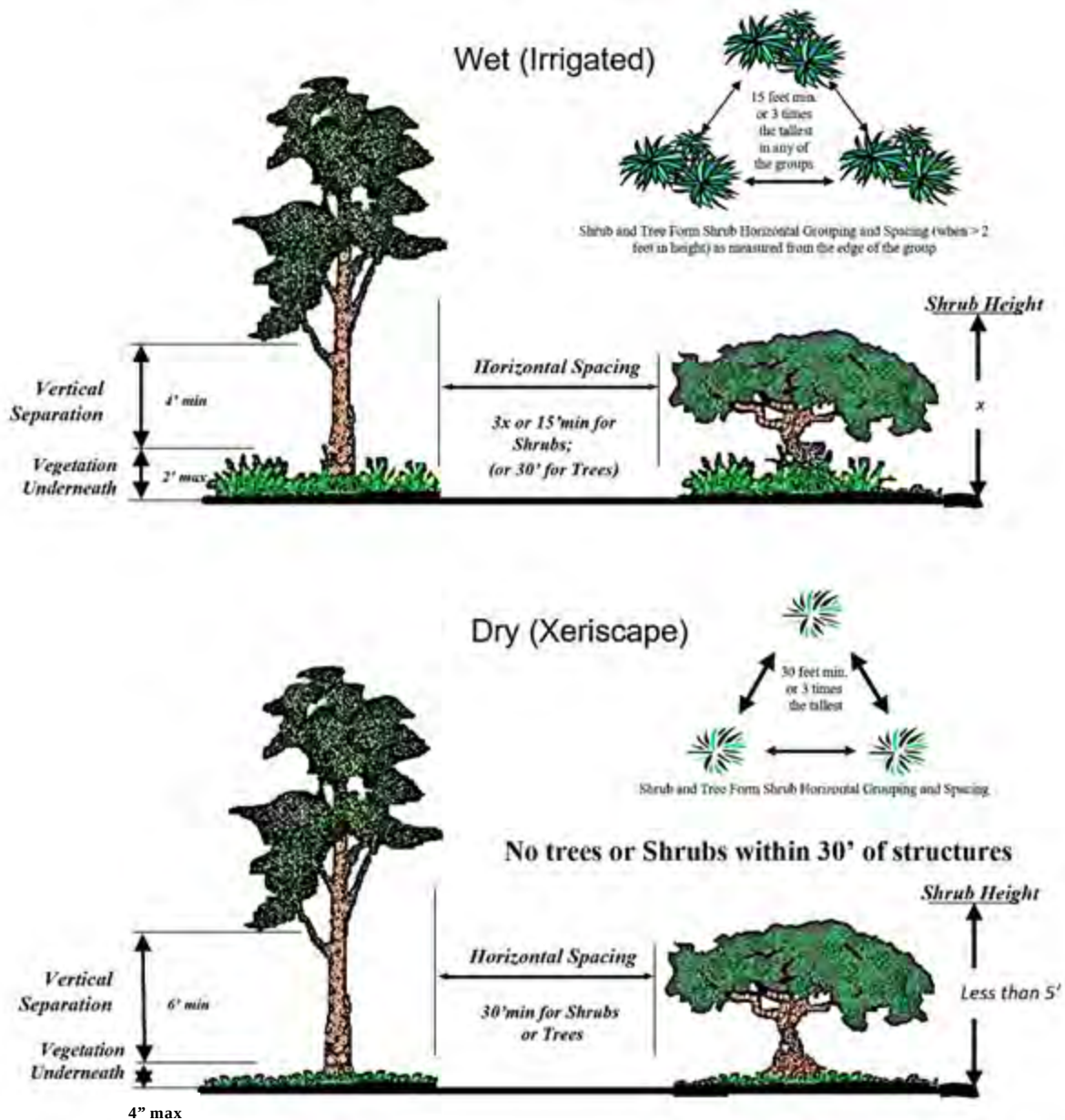
Figure 41 – Zone 1 Horizontal and Vertical Spacing/Separation Requirements
