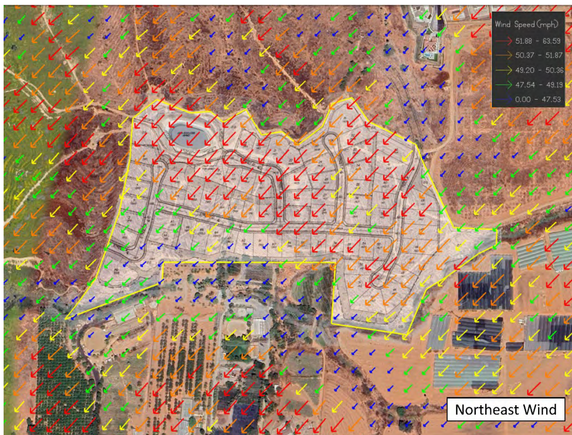
Figure 23 – Northeast Wind
