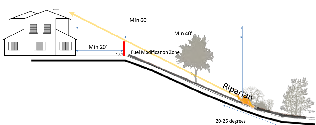
Figure 39 – Radiant Heat Wall Orientation
