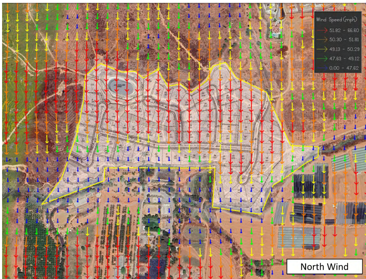
Figure 22 – North Wind
