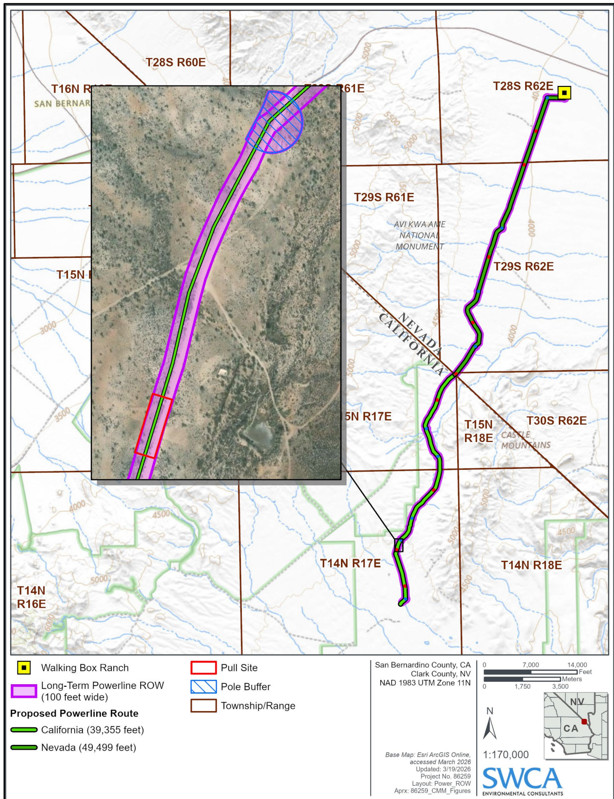
Figure 2-6. 69-kV Overhead Power Line Location under the Proposed Action
