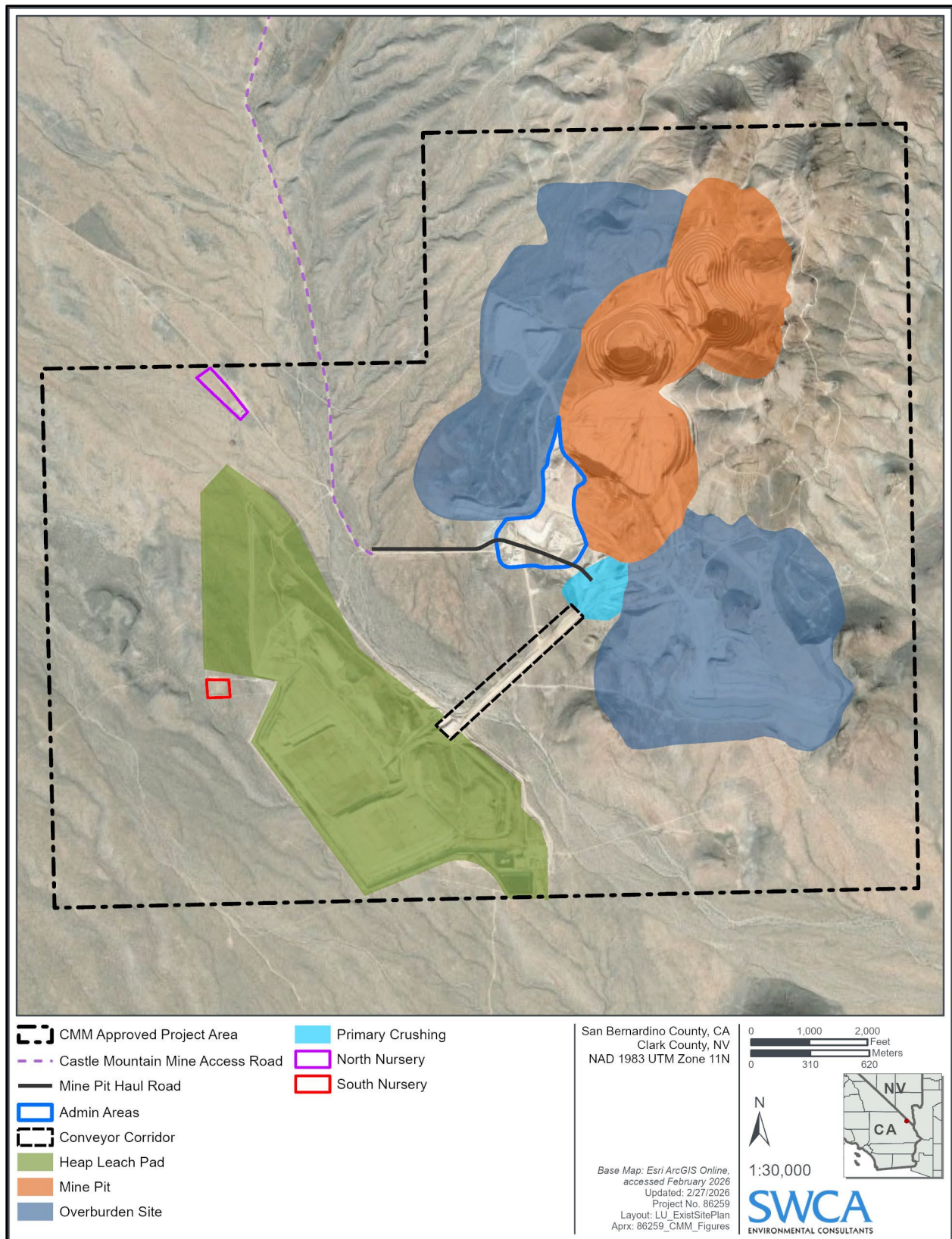
Figure 2-1. No Action Alternative Map
