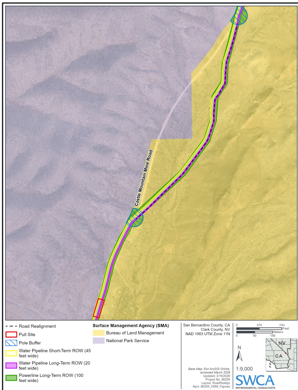
Figure 2-4. Proposed Administrative Access Road Segment
