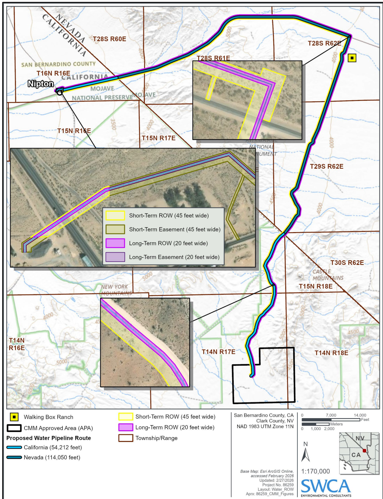
Figure 2-5. Underground Water Pipeline Location under the Proposed Action
