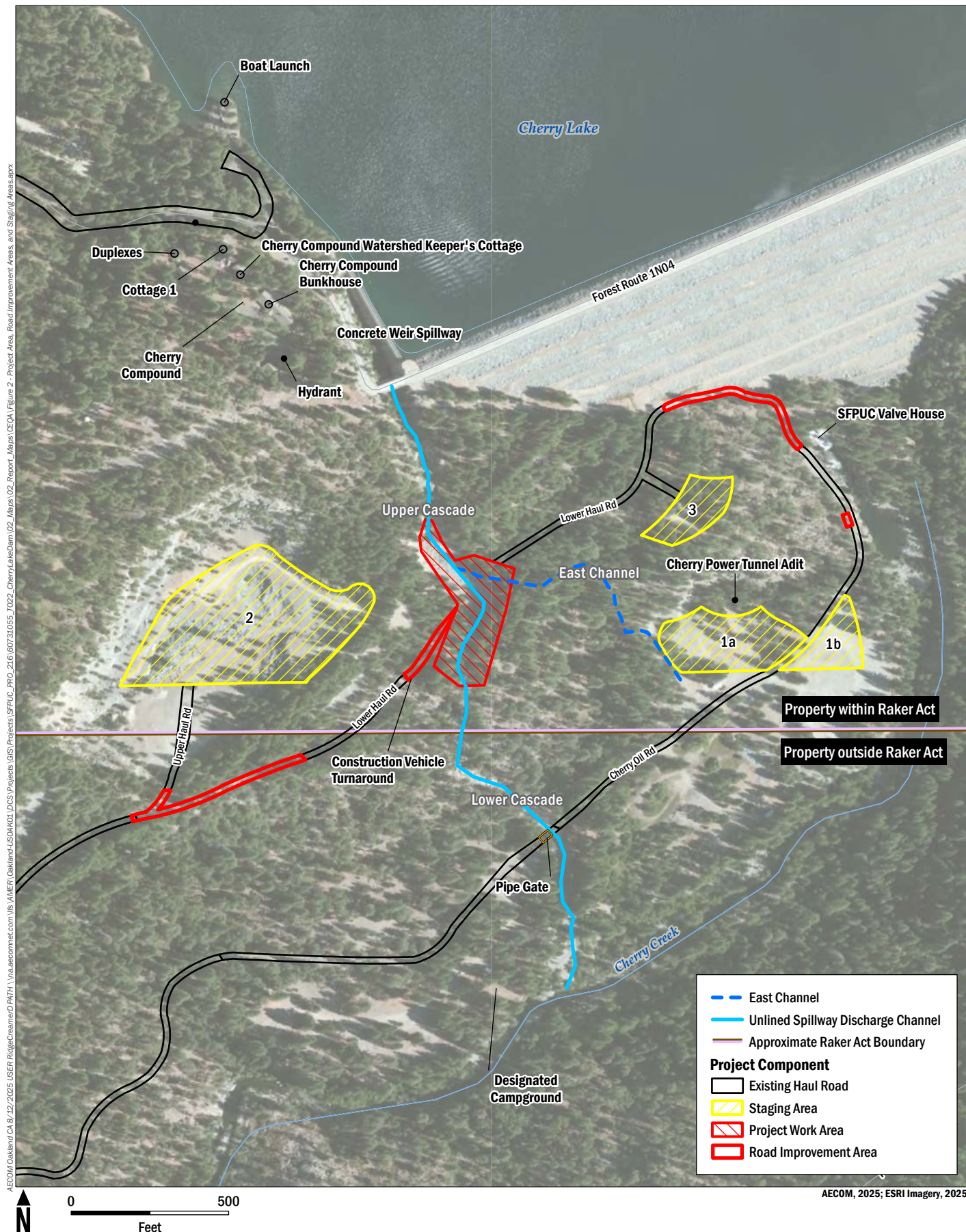
FIGURE 2 Project Area, Road Improvement Areas, and Staging Areas
