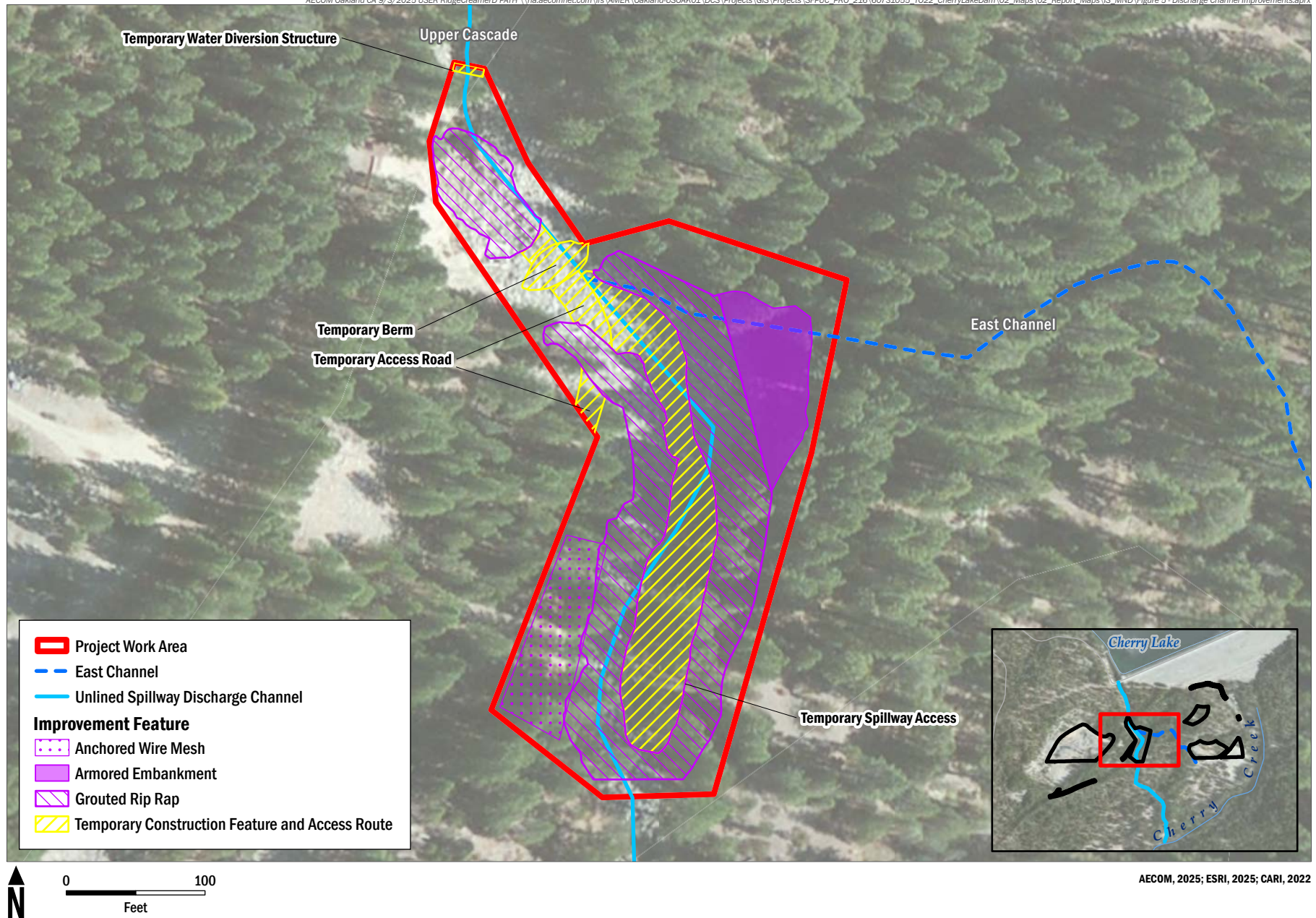
FIGURE 5 Discharge Channel Improvements
