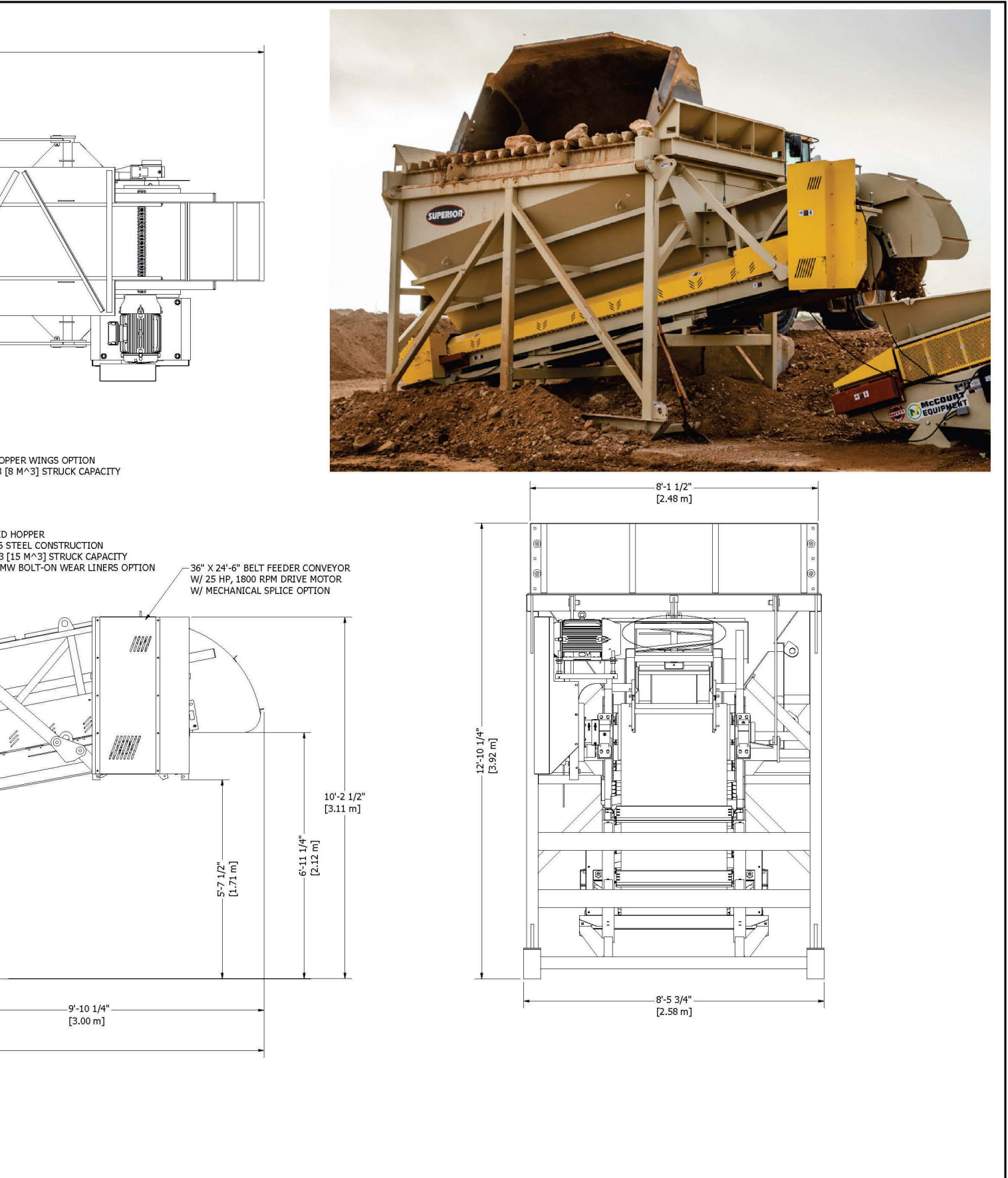
Figure 2-11 Proposed Skid-Mounted Feed Hopper
