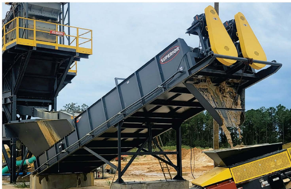
Figure 2-13 Proposed Twin Fine-Material Washers Sand Screw
