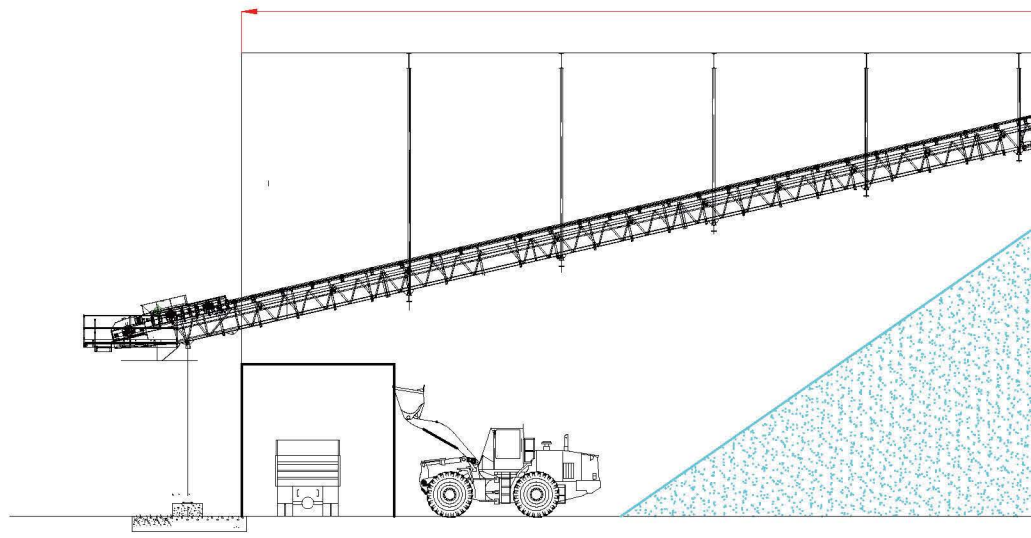
2 VIEW B-B - WAREHOUSE SIDE VIEW
