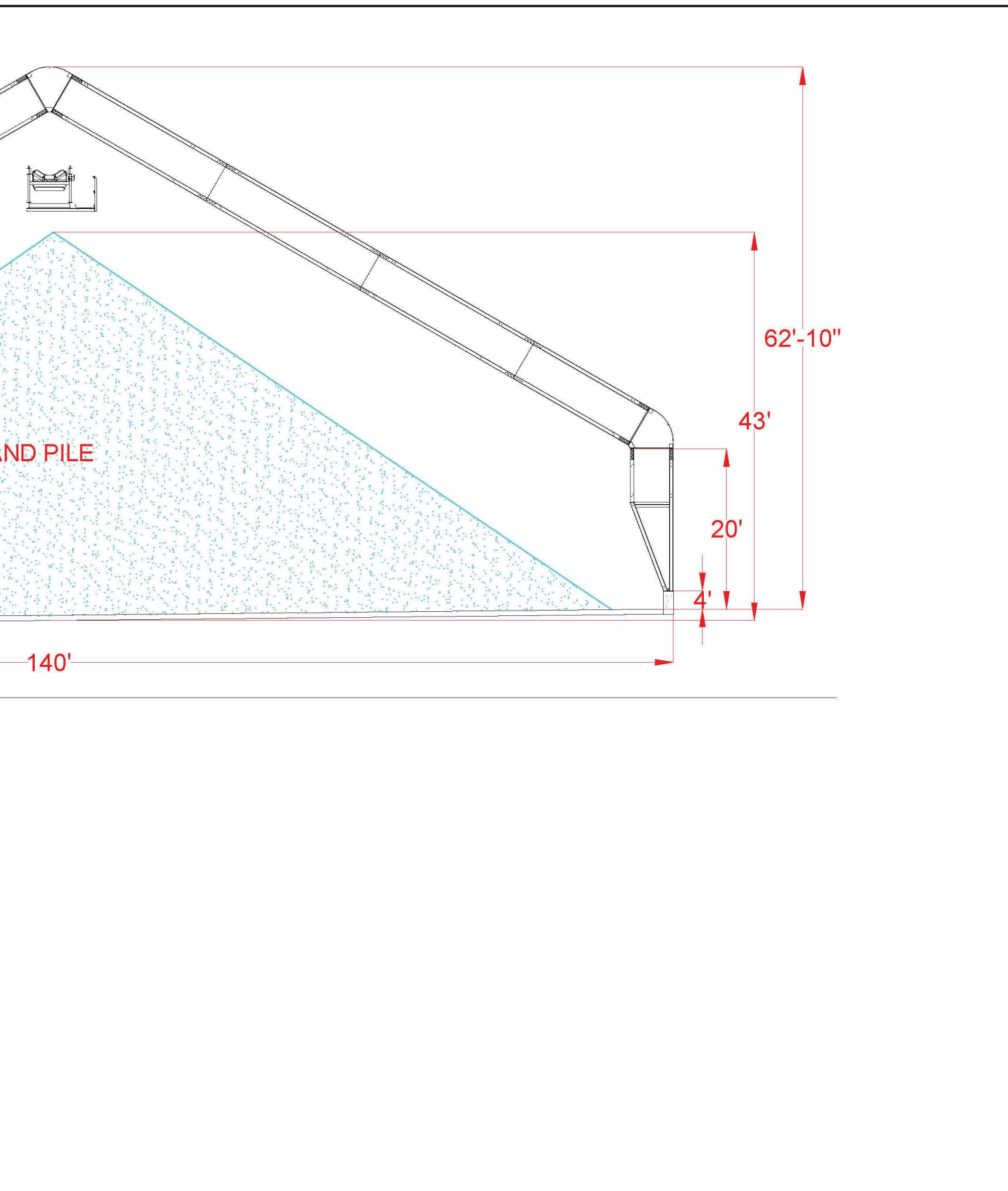
Figure 2-6 Proposed Storage Warehouse (front view)
