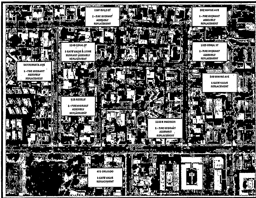
Coral Gate Valve Vicinity Map
