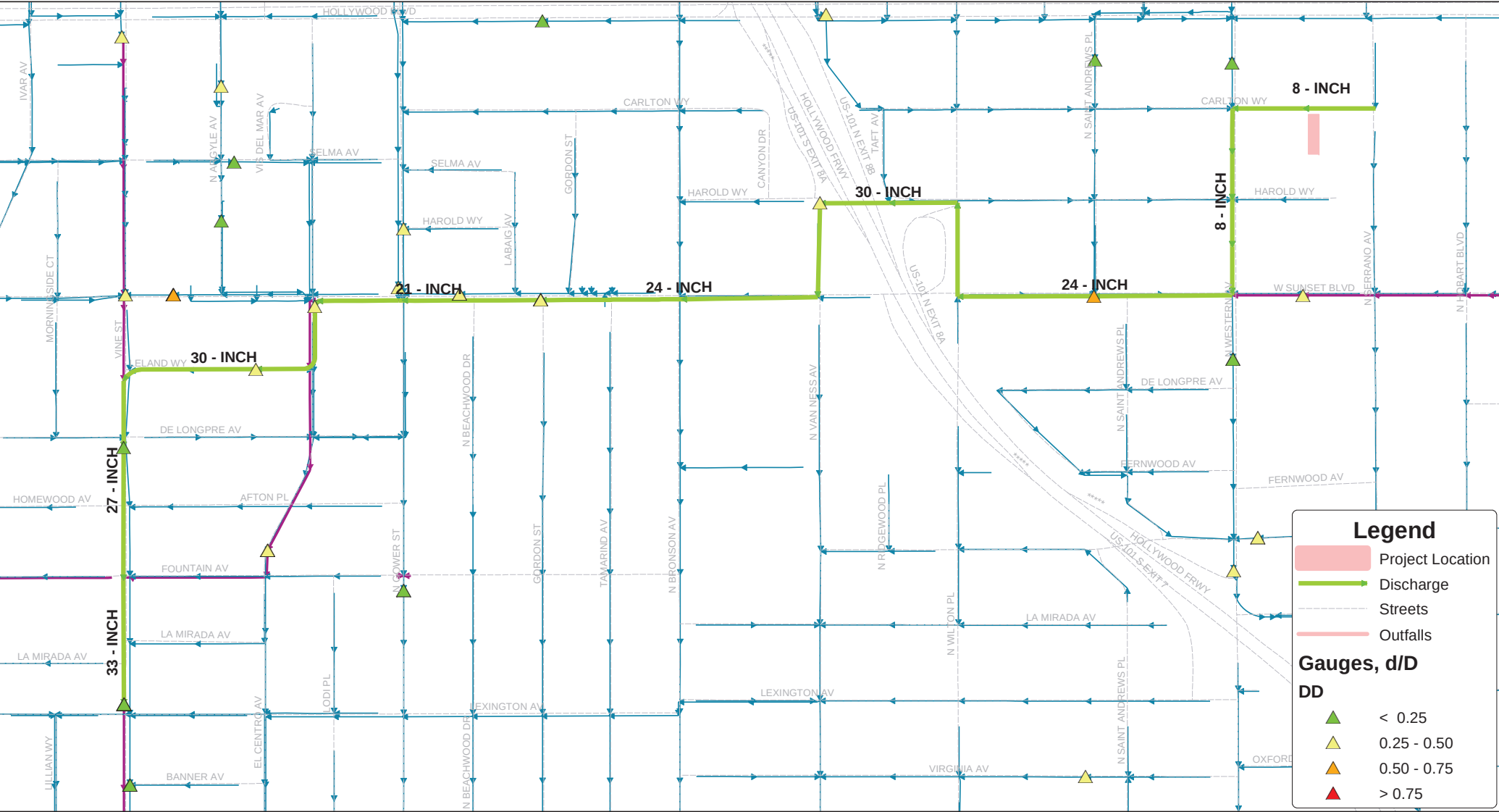
Figure 1 5424 Carlton Way Project Sewer Map
