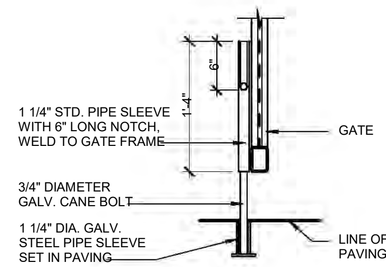
5 LATCH DETAIL 1" = 1'-0"
