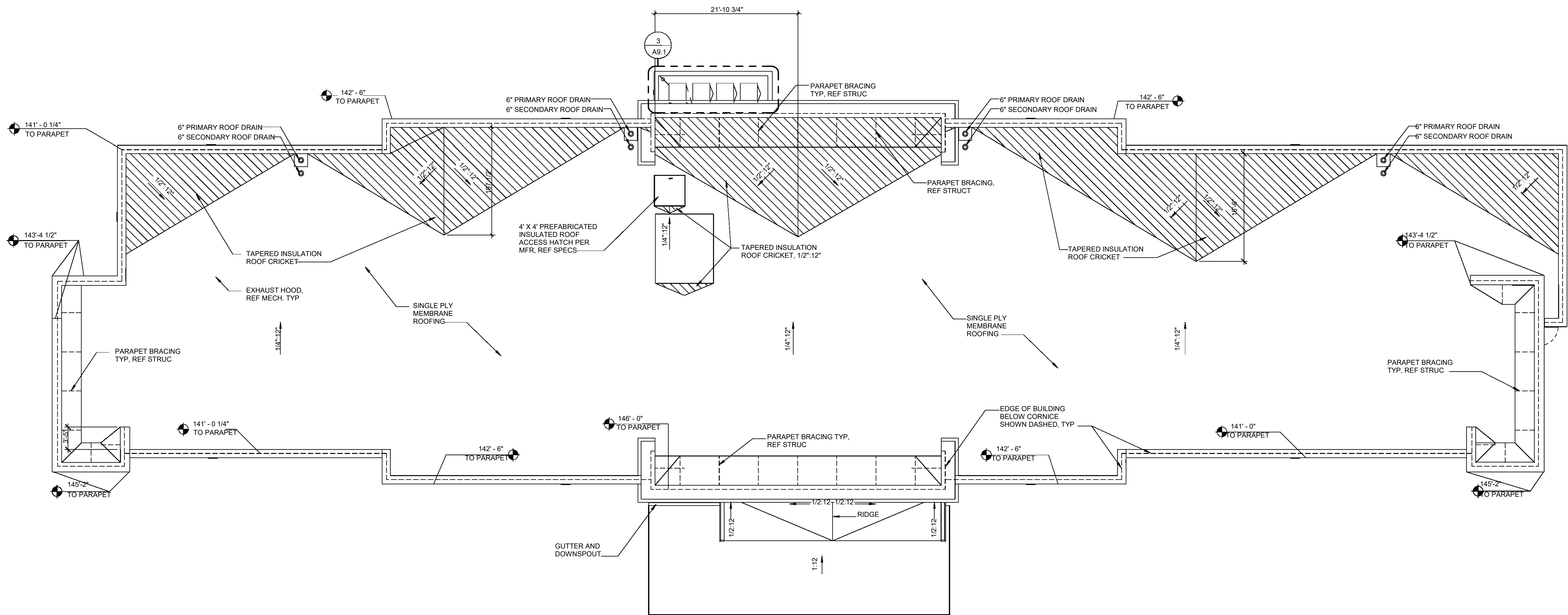
1 ROOF PLAN 1/8" = 1'-0"
