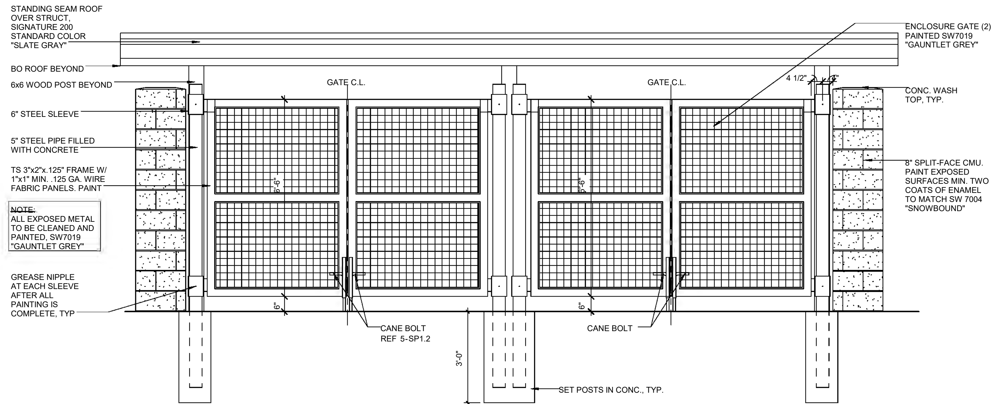
6 TRASH ENCLOSURE GATE ELEVATION 1/2" = 1'-0"
