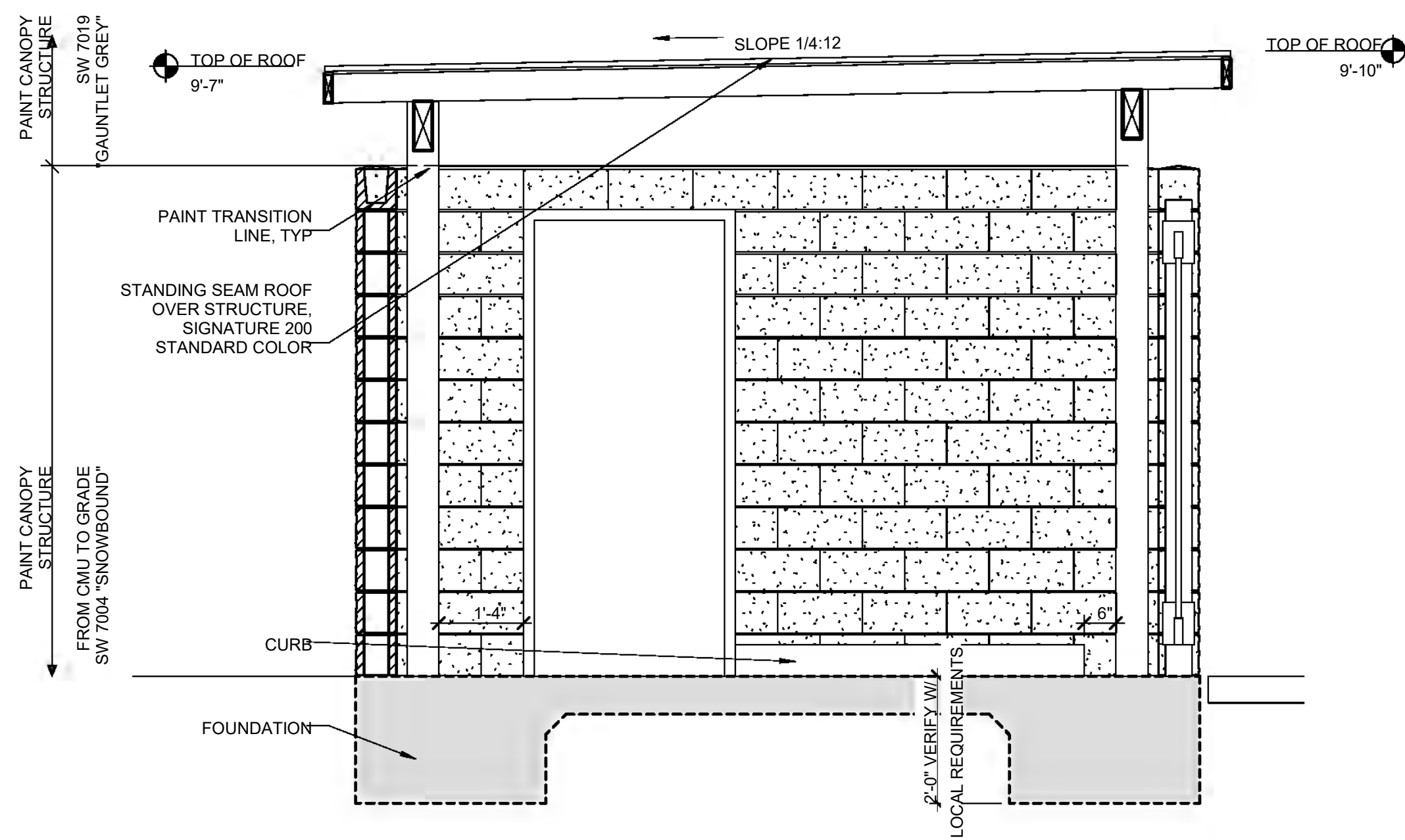
7 TRASH ENCLOSURE GATE SECTION 1/2" = 1'-0"
