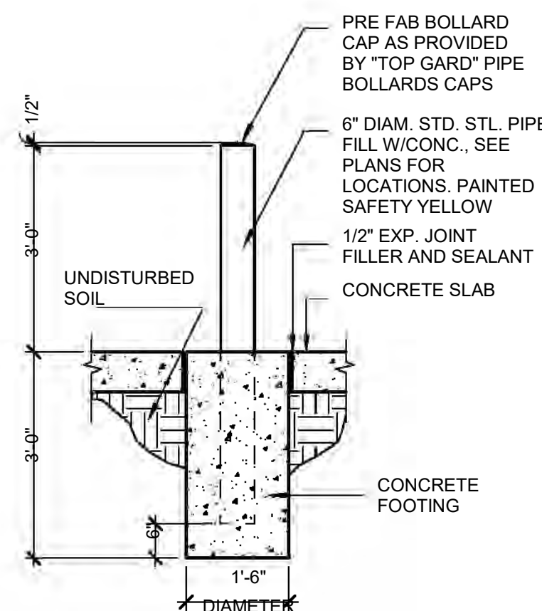
3 PIPE BOLLARD 1/2" = 1'-0"
