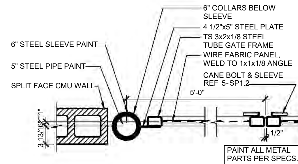
4 SECTION THROUGH GATE 1" = 1'-0"
