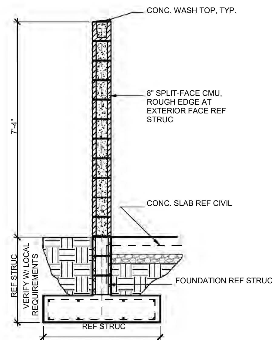
2 TRASH ENCLOSURE WALL SECTION 1/2" = 1'-0"
