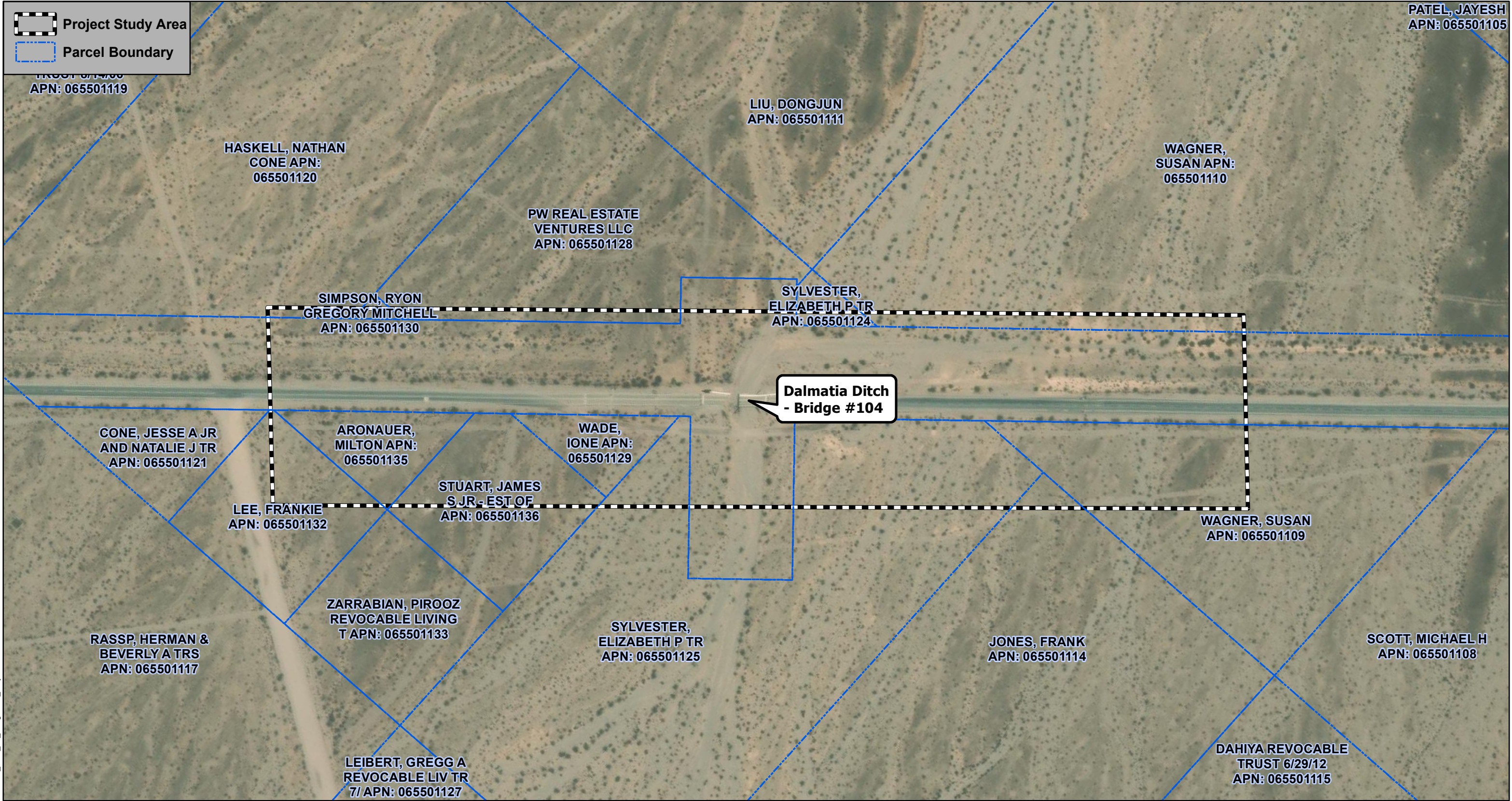
Figure 3 Page 11 of 19 Project Features - Dalmatia Ditch 54C0308 HBP-5954 (168-186) National Trails Highway at 19 Bridges Project San Bernardino County, California
