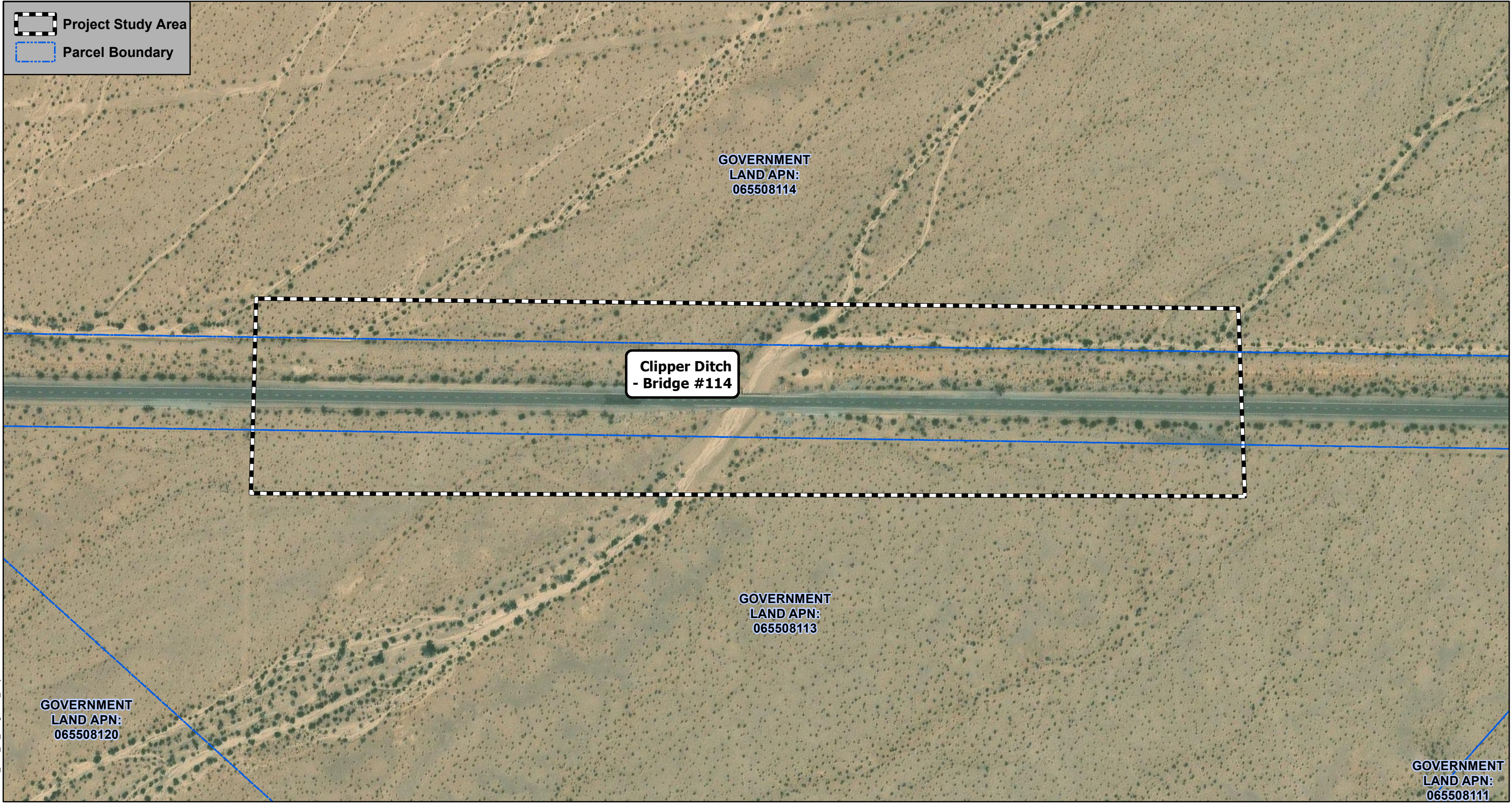
Figure 3 Page 16 of 19 Project Features - Clipper Ditch 54C0318 HBP-5954 (168-186) National Trails Highway at 19 Bridges Project San Bernardino County, California
