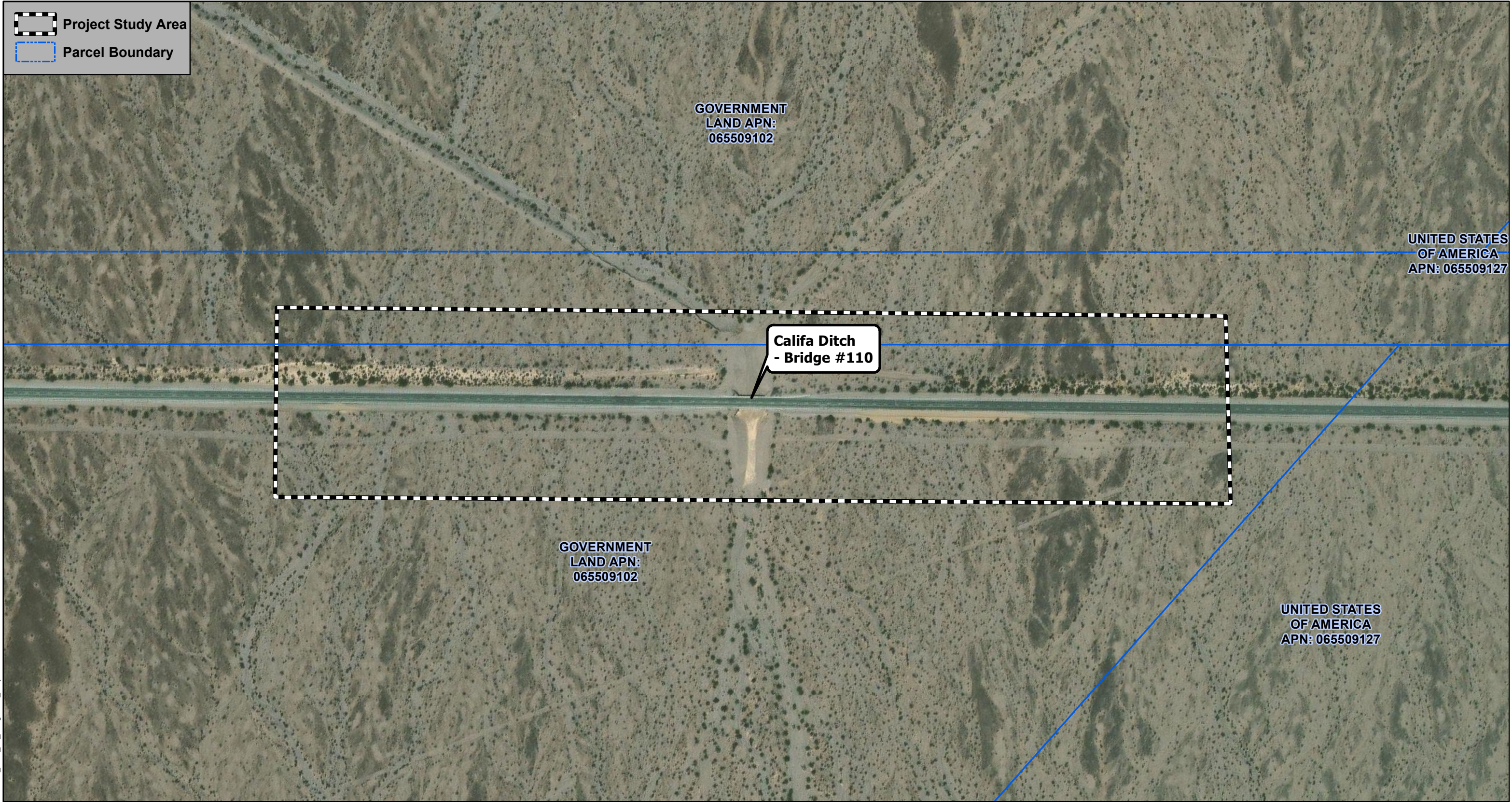
Figure 3 Page 15 of 19 Project Features - Califa Ditch 54C0314 HBP-5954 (168-186) National Trails Highway at 19 Bridges Project San Bernardino County, California
