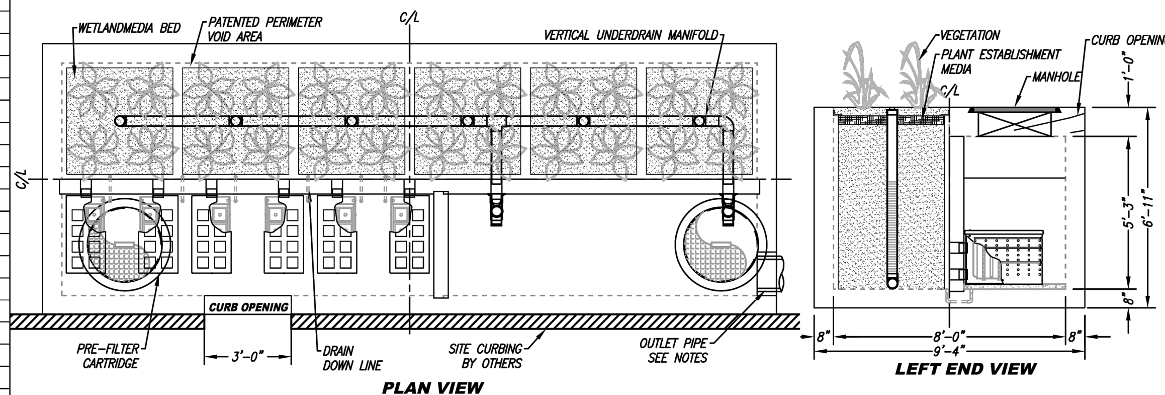
PLAN VIEW
