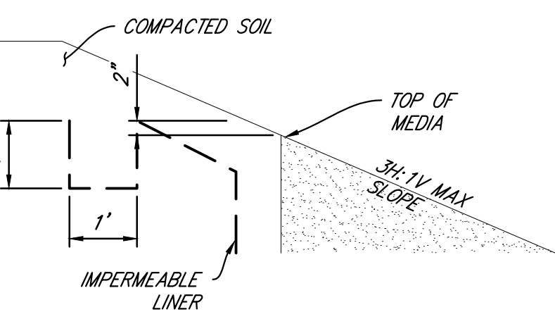
IMPERMEABLE LINER EDGE ANCHOR DETAIL NOT TO SCALE
