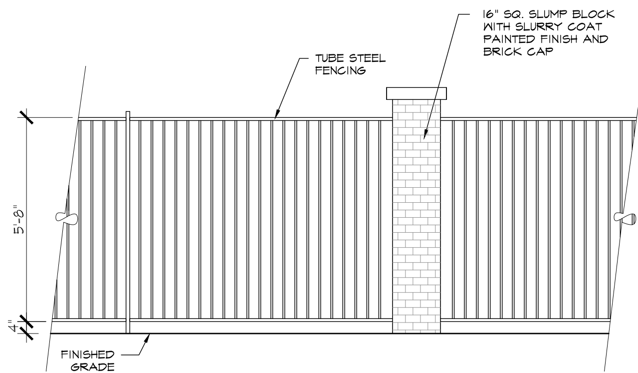
D SIDEYARD FENCING AND PILASTER
