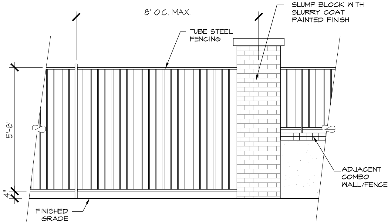
A TUBE STEEL FENCING
