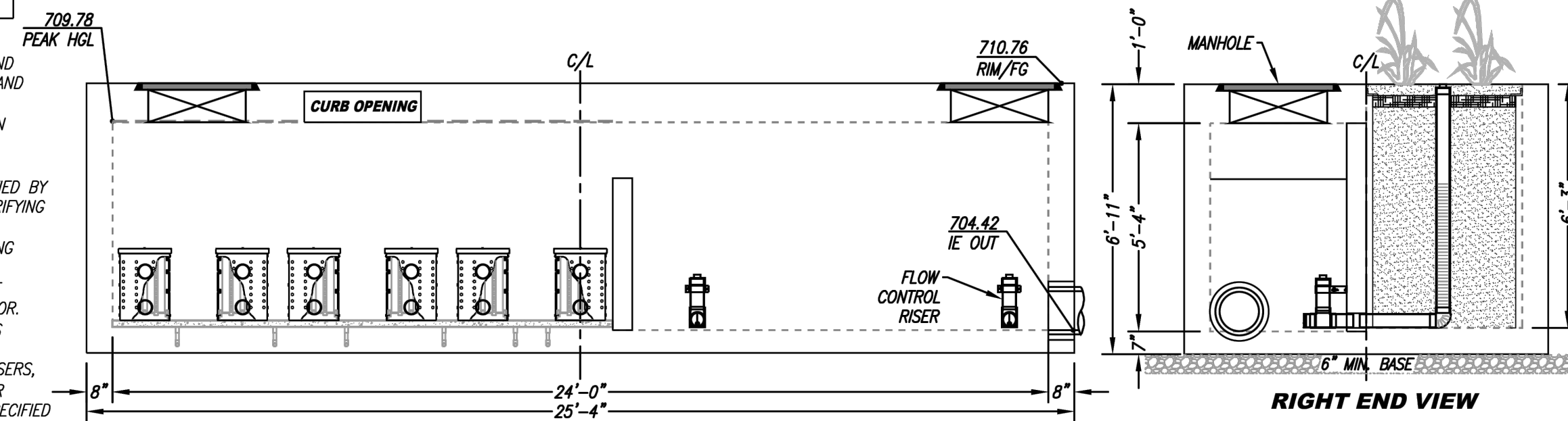
ELEVATION VIEW
