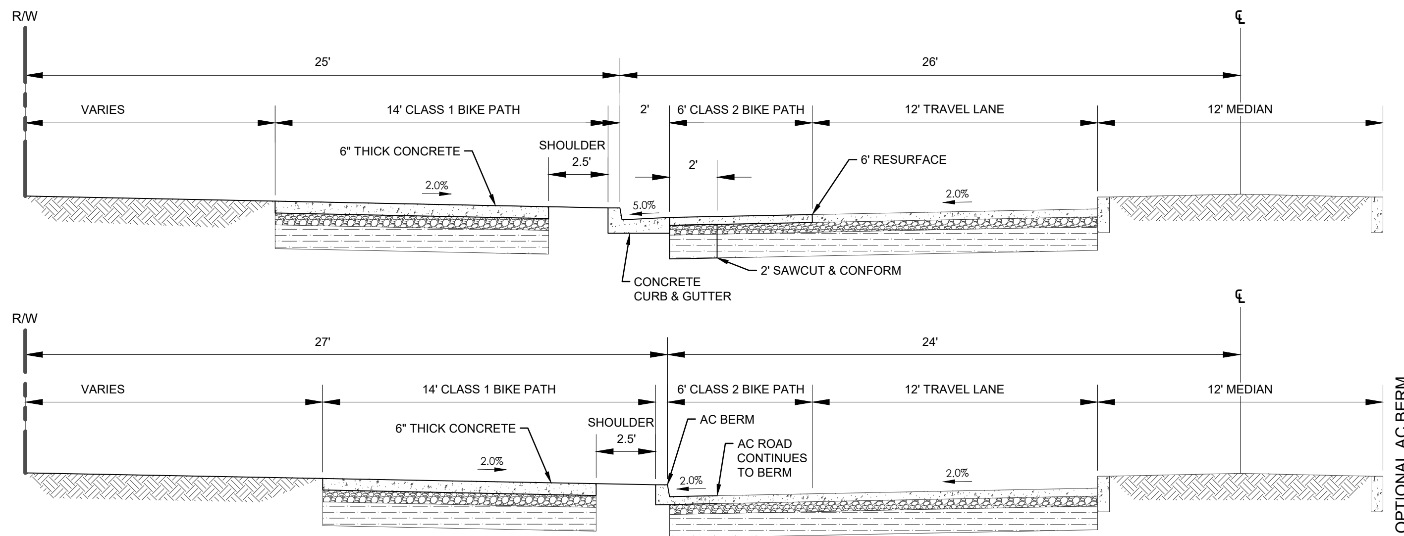
SECTION A-A HOLLISTER AVENUE SCALE: 1"=4'
