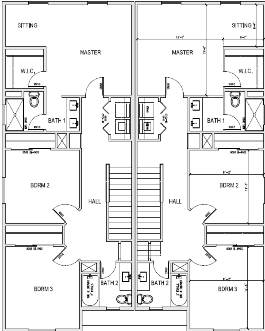
Plan 1481 2nd Floor - 934 s.f. 1/8" = 1'-0"
