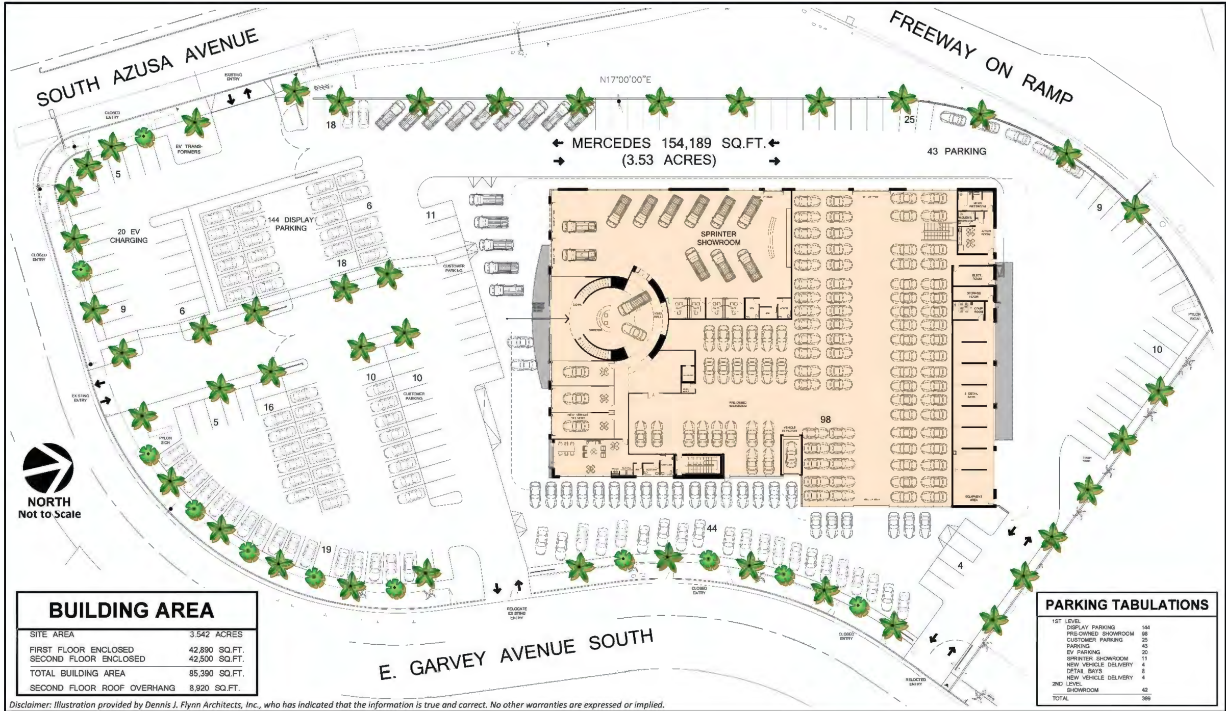
Figure 3.4-1 SITE PLAN
