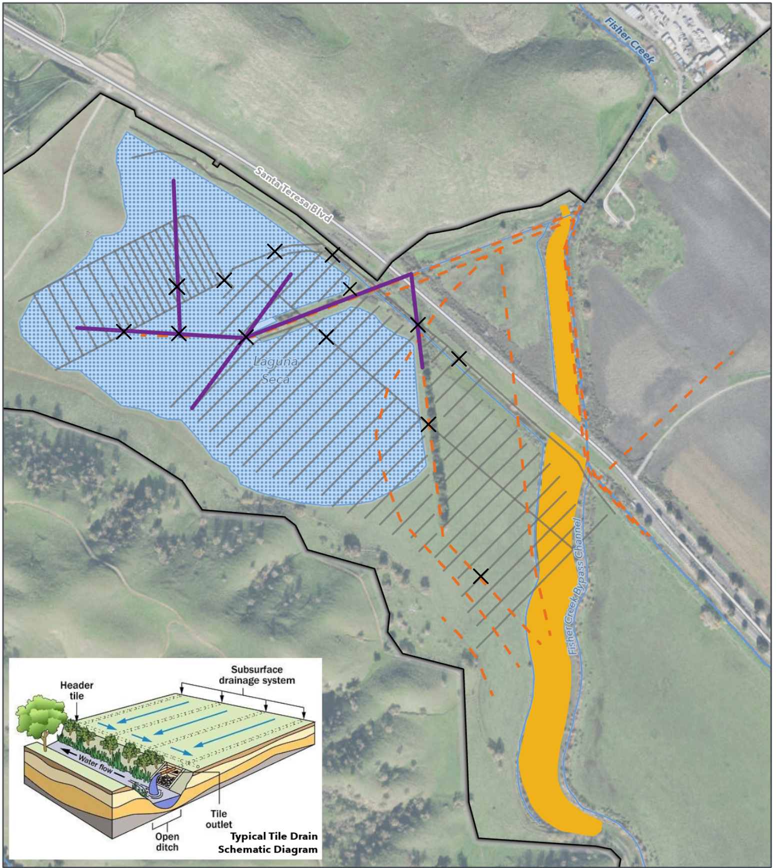
Figure 3: Laguna Seca Existing Drainage Infrastructure
