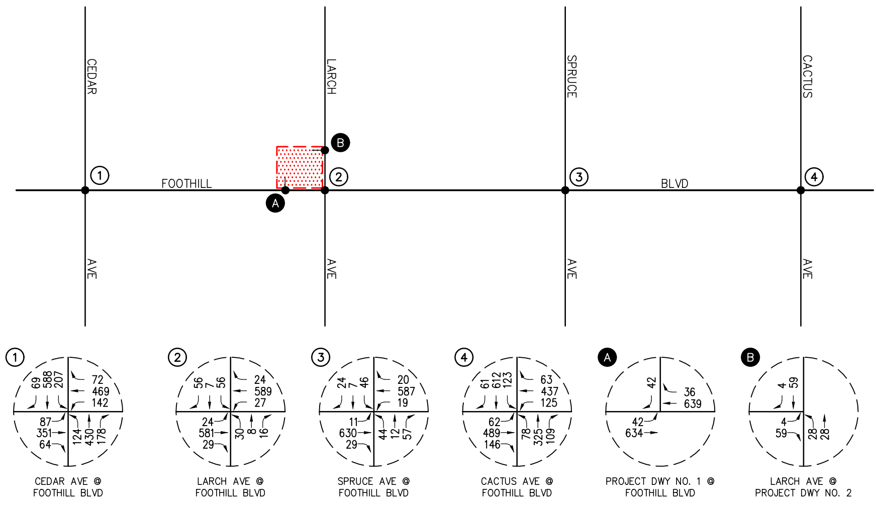
FIGURE 6-1 EXISTING WITH PROJECT AM PEAK HOUR TRAFFIC VOLUMES FOOTHILL AND LARCH CHICK-FIL-A, RIALTO
