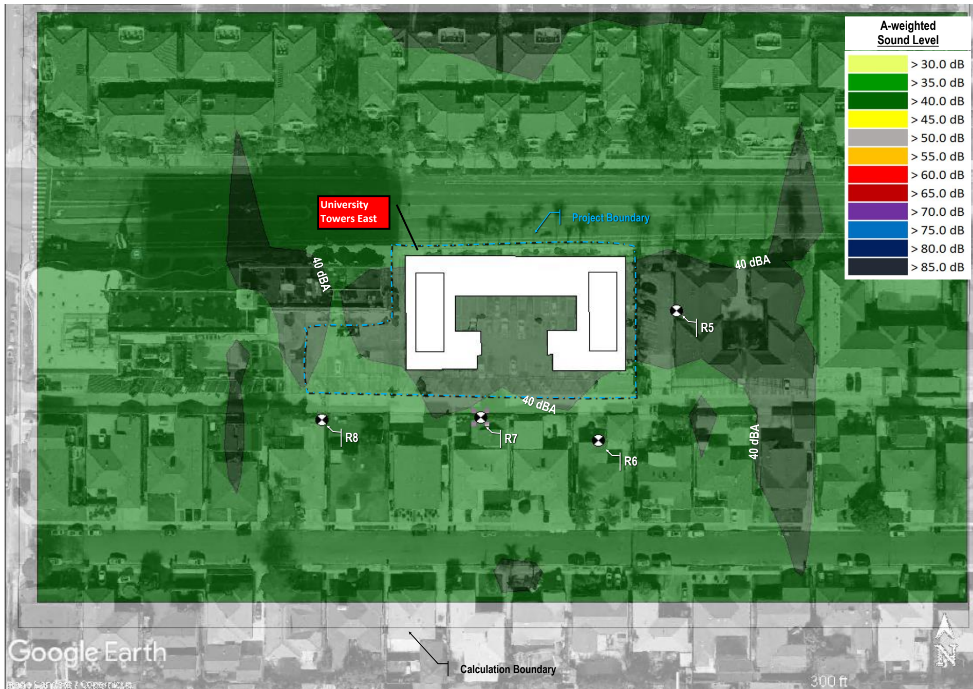
FIGURE 5 Predicted Stationary Source Operation Noise from Proposed Project (University Towers East Component)
