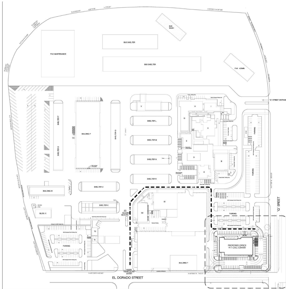
OVERALL SITE KEY PLAN SCALE: 1"=60'-0"
