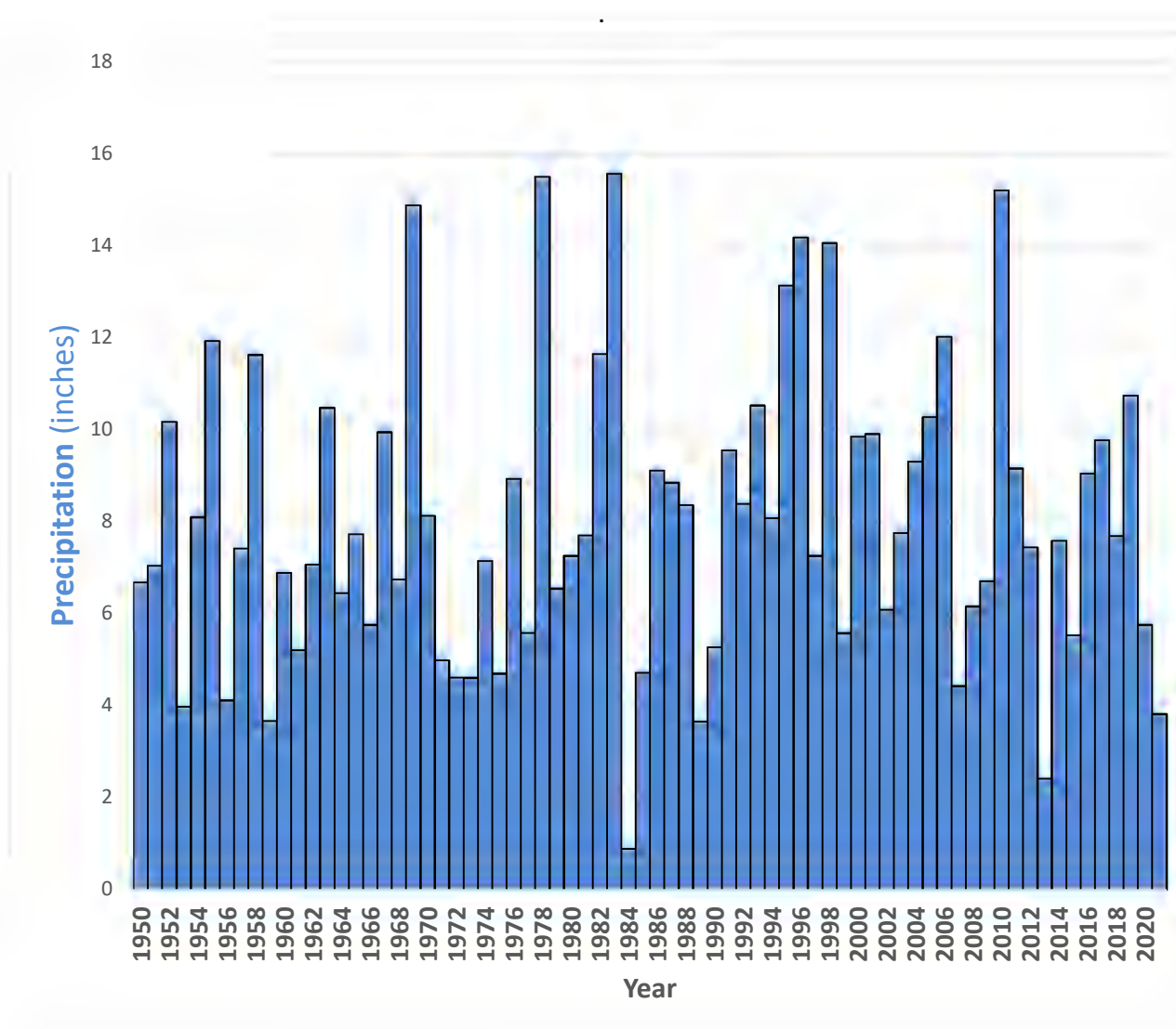
Figure 3-5 Historical Annual Rainfall
