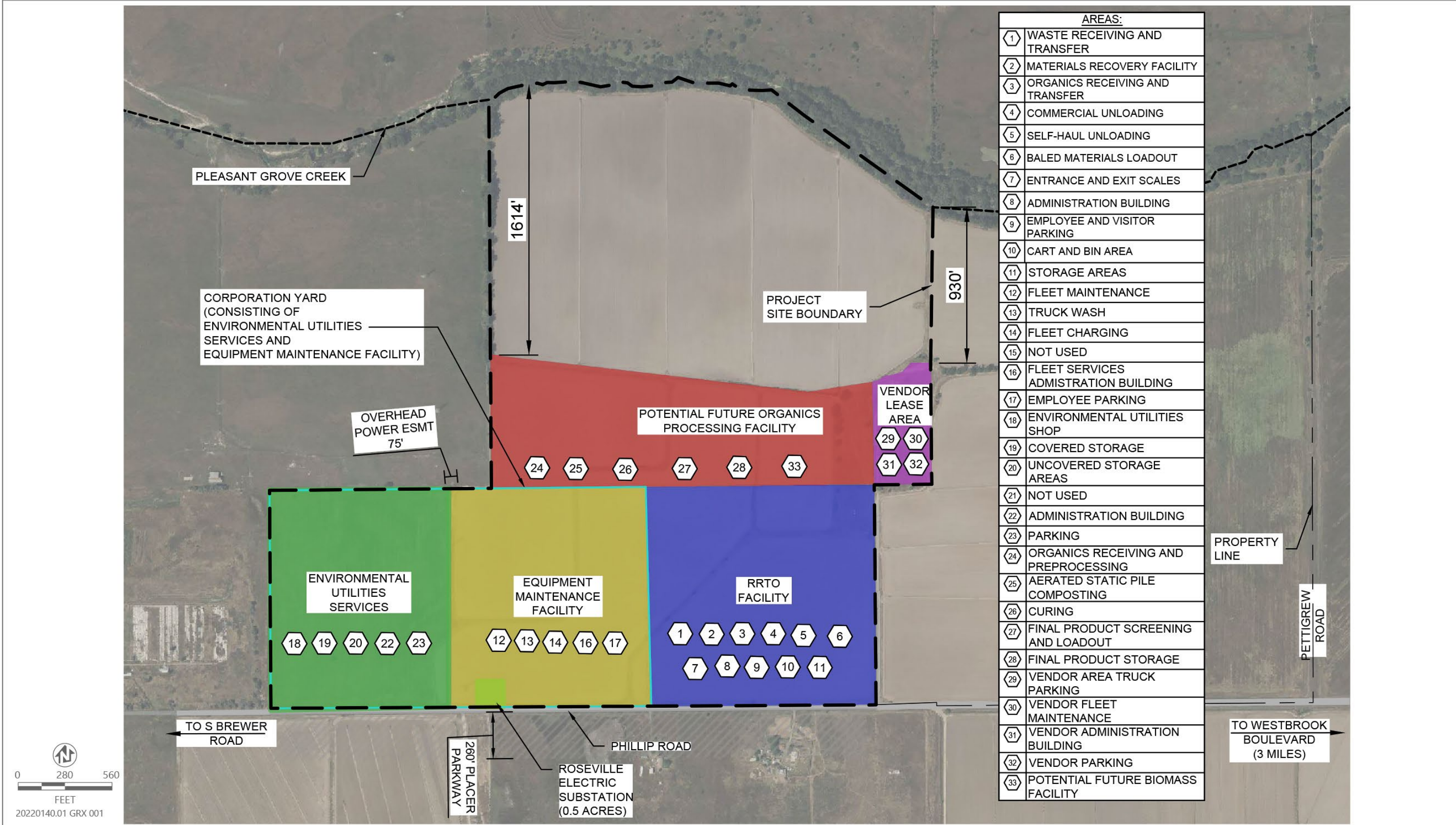
Figure 2-3 Proposed Services/Facilities Areas
