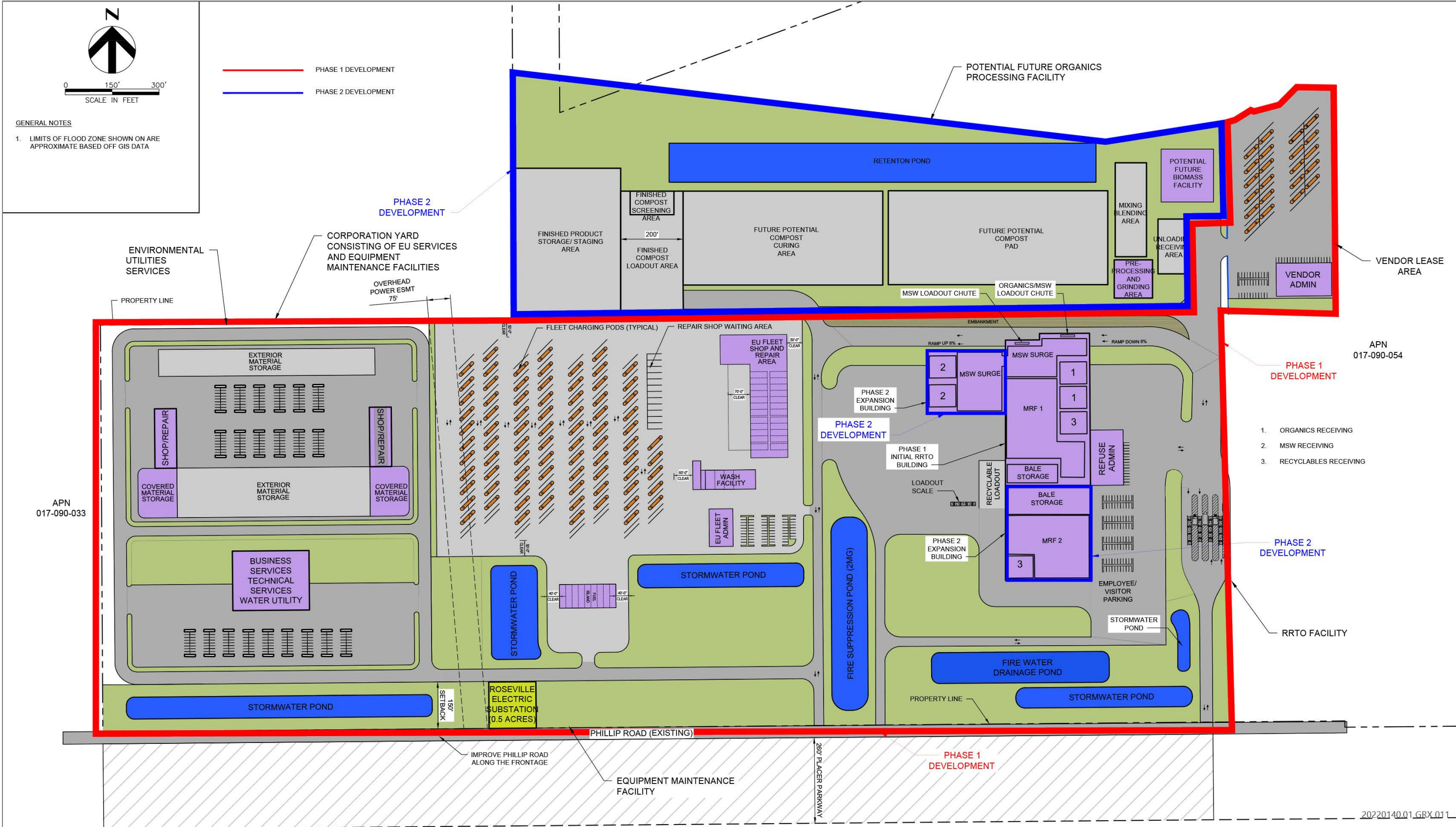
Figure 2-5 Proposed Phasing Plan
