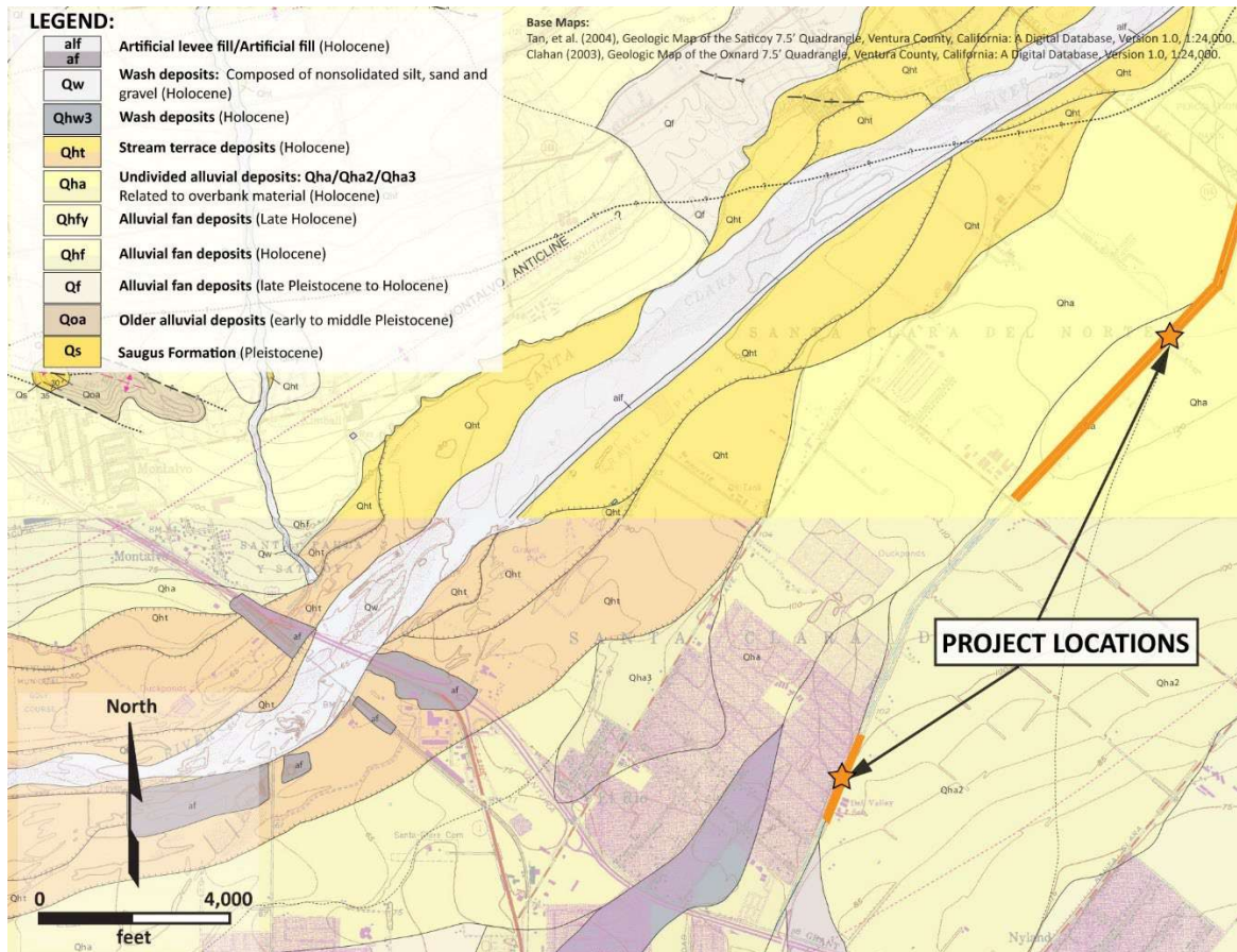
Figure 2: Geologic Map (Tan, et al. 2004, Clahan 2003)
