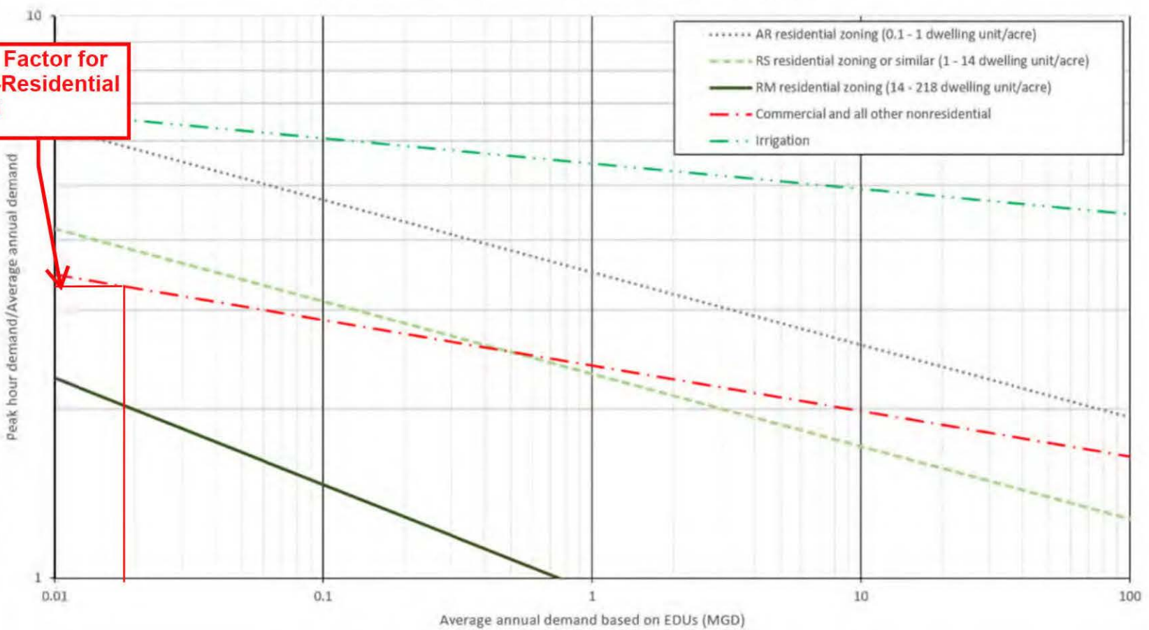
Figure 2-1 Peak-Hour Demand Factor by Development Type and Size
