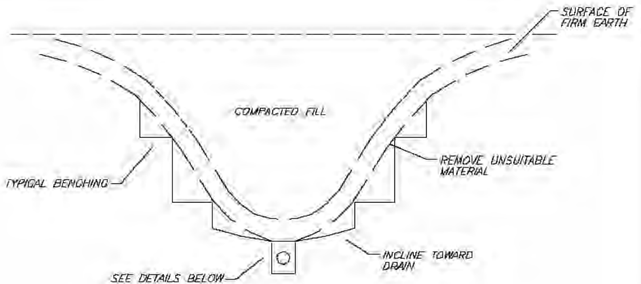
TRENCH DETAIL
