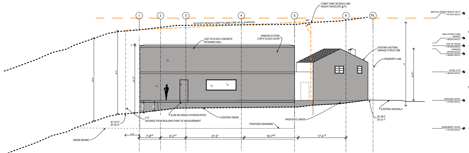
SOUTH ELEVATION
