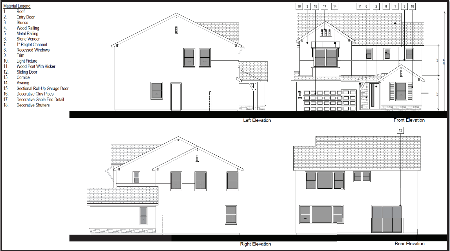
Figure 14c: Conceptual Residential Elevations
