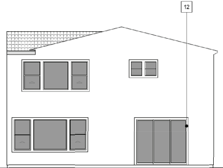
Rear Elevation
