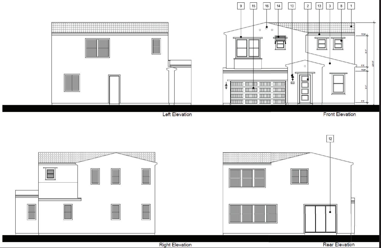
Figure 12a: Conceptual Residential Elevations
