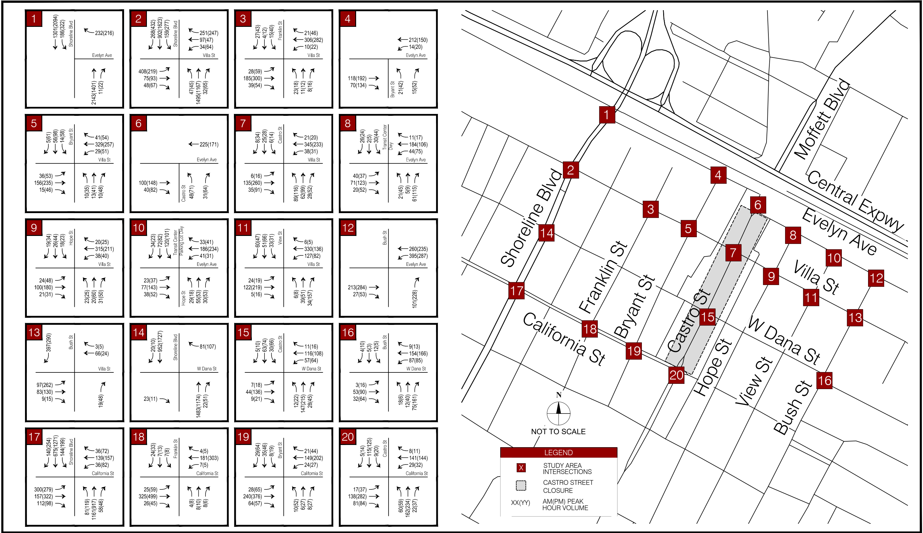
FIGURE 1 BASELINE AM AND PM PEAK HOUR TURNING MOVEMENT VOLUMES CASTRO PEDESTRIAN MALL FEASIBILITY STUDY
