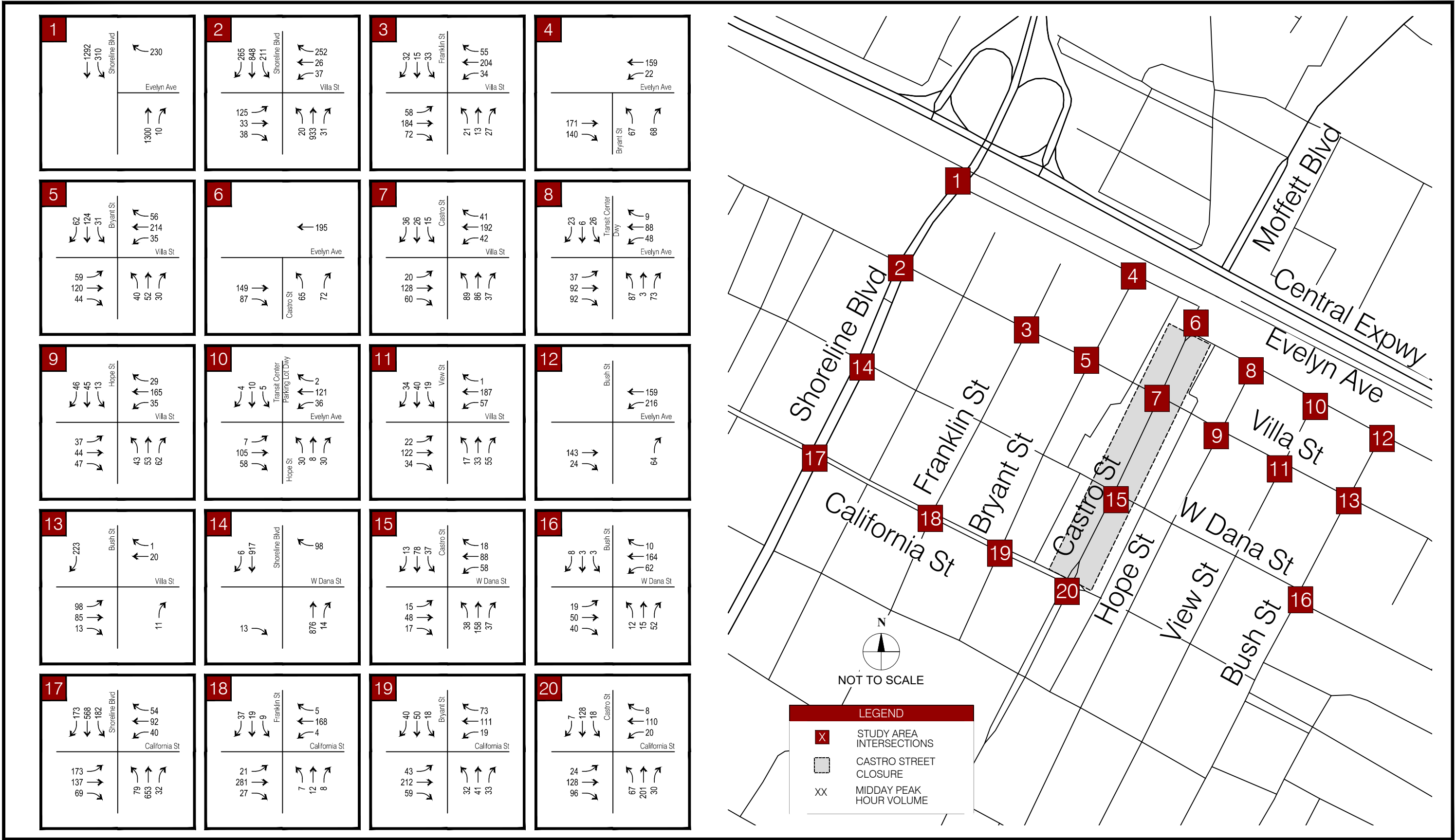
FIGURE 2 BASELINE MIDDAY PEAK HOUR TURNING MOVEMENT VOLUMES CASTRO PEDESTRIAN MALL FEASIBILITY STUDY
