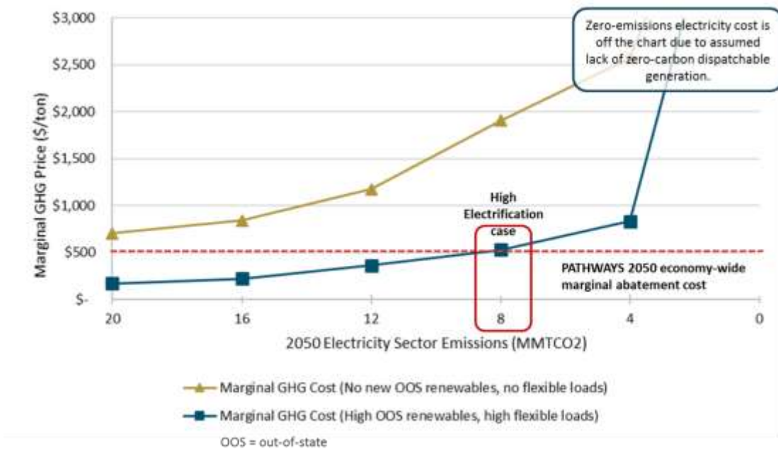
Figure 15: 2050 Marginal Electricity Sector GHG Abatement Cost
