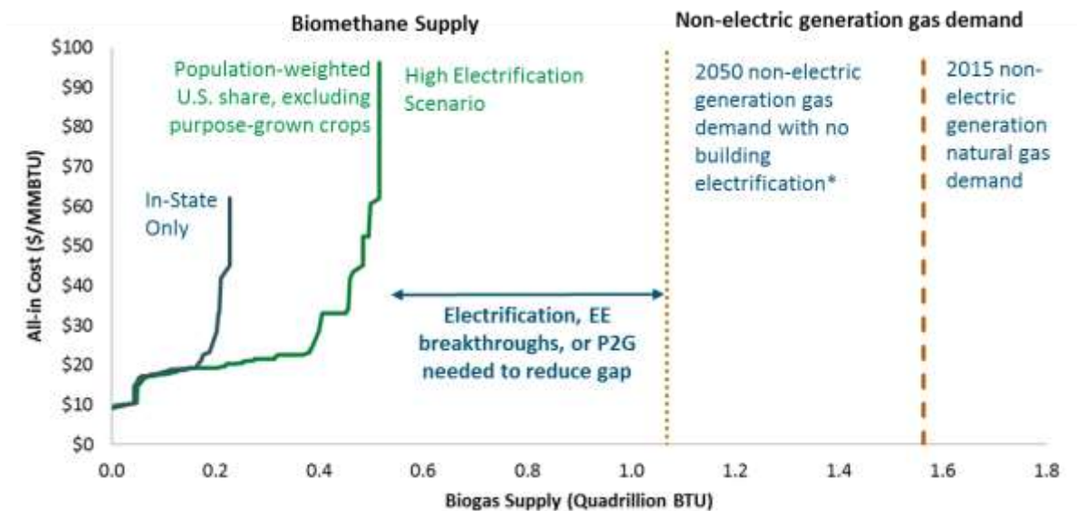
Figure 9: Estimated Cost and Available Biomethane Supply to California in 2050 Compared with Non-Electric Natural Gas Demand
