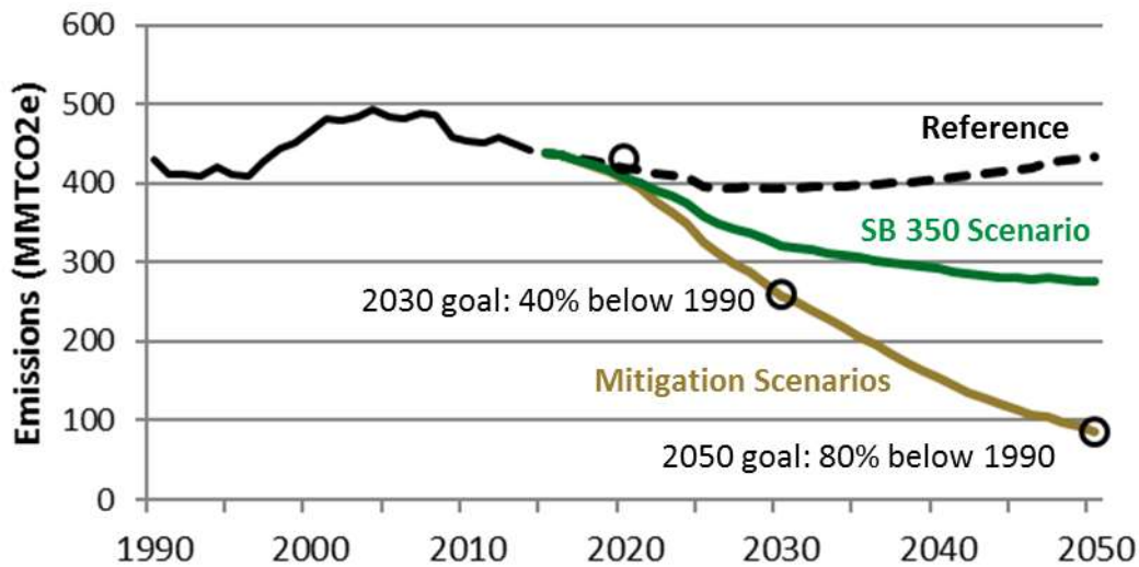
Figure 5: California Greenhouse Gas Emissions by Scenario
