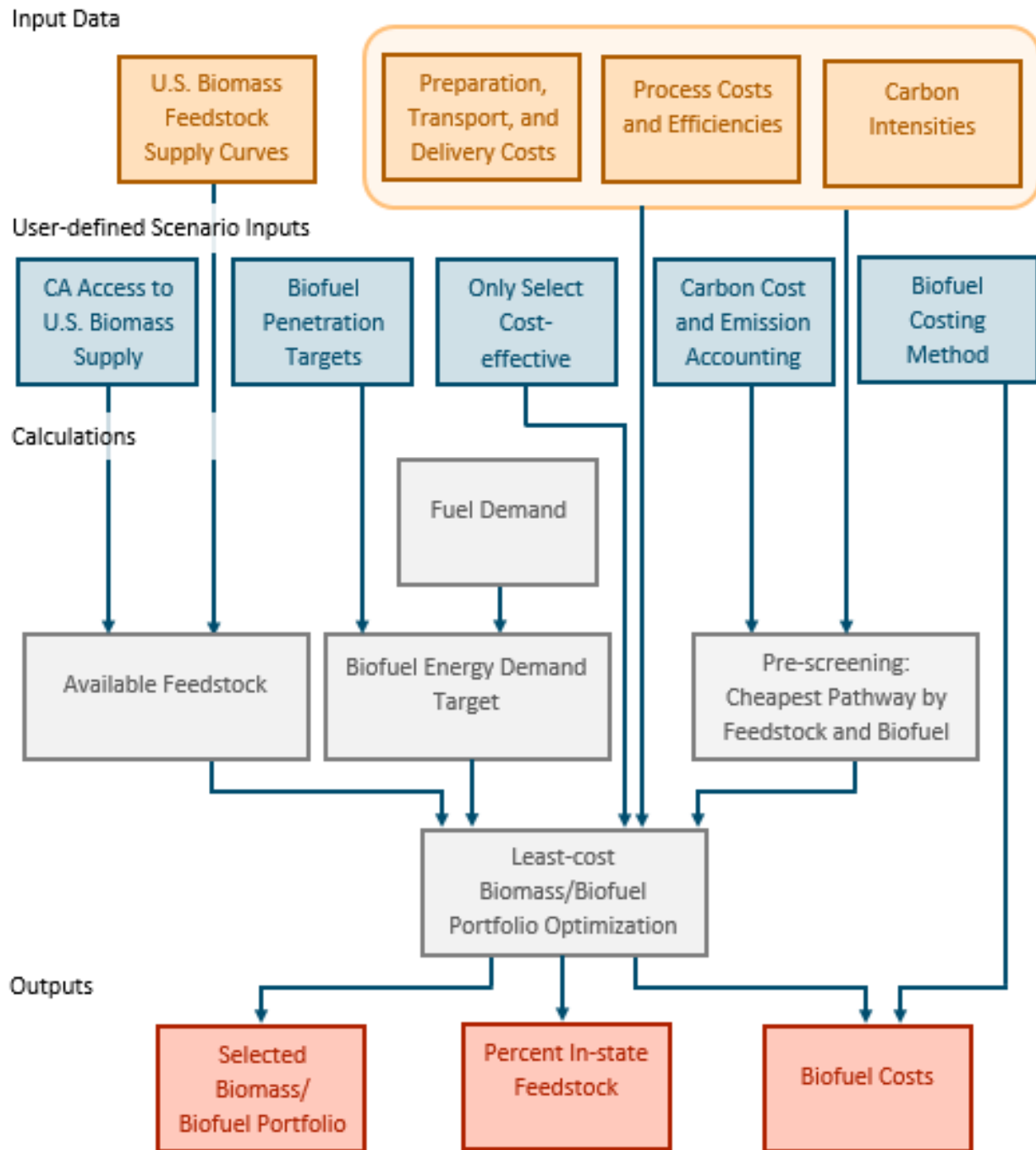
Figure C-1: Cost Minimization Biofuel Module Flow Chart
