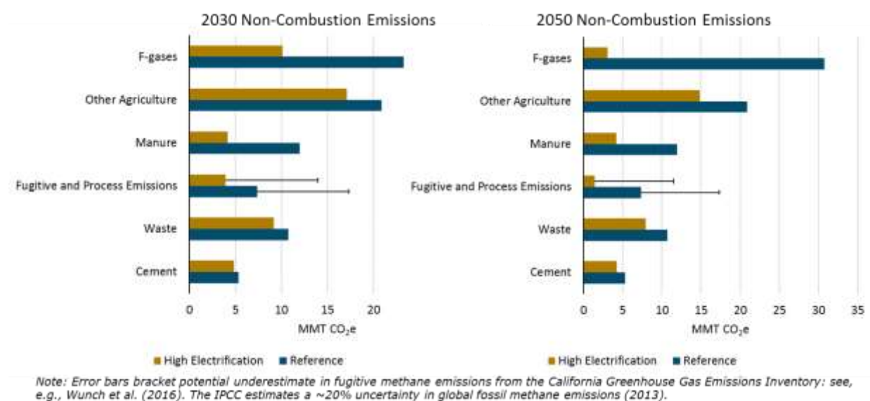
Figure 21: Non-combustion Emissions in 2030 and 2050 in the Reference and High Electrification Scenario
