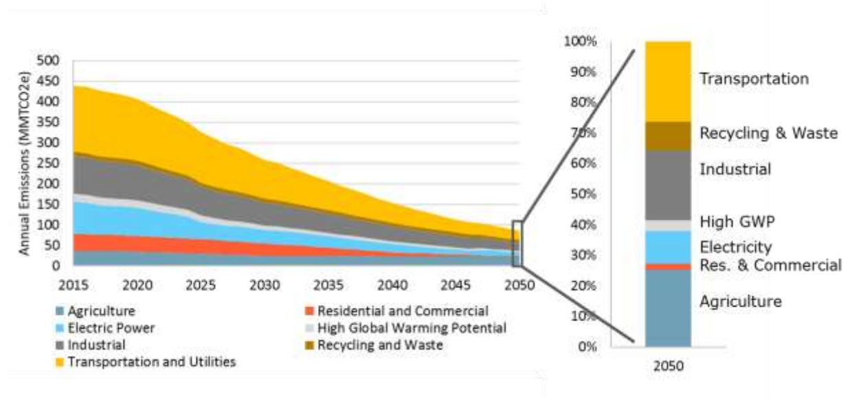
Figure 6: California Greenhouse Gas Emissions by Sector in the High Electrification Scenario
