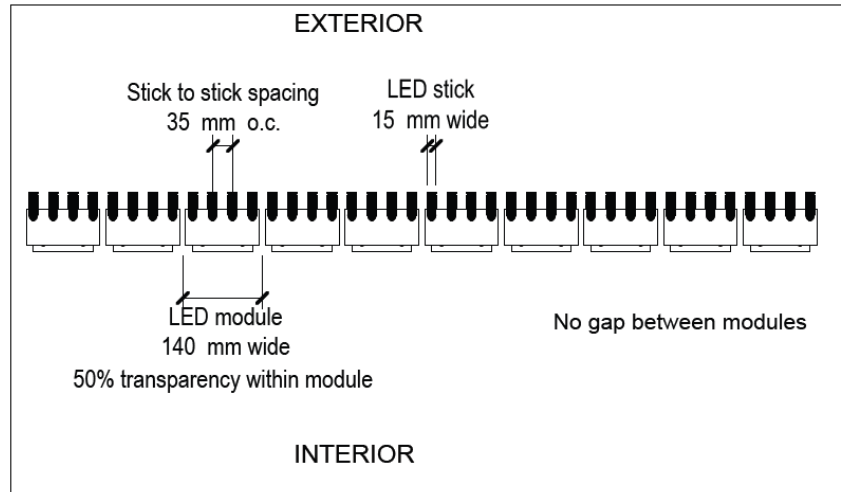
PRIMARY ADVERTISING AREA STRUCTURAL PLAN
