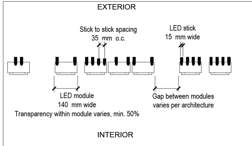
INTEGRATION AREA STRUCTURAL PLAN
