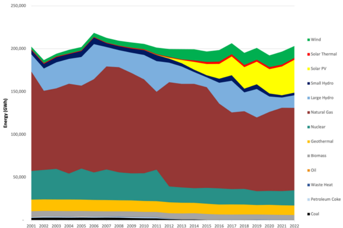
FIGURE 5-1. IN-STATE ELECTRIC GENERATION BY FUEL TYPE (2011-2022)
