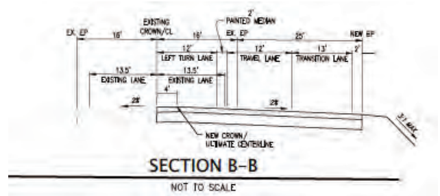
Figure 3-3 PROPOSED ENTRY IMPROVEMENTS ON MARIPOSA ROAD
