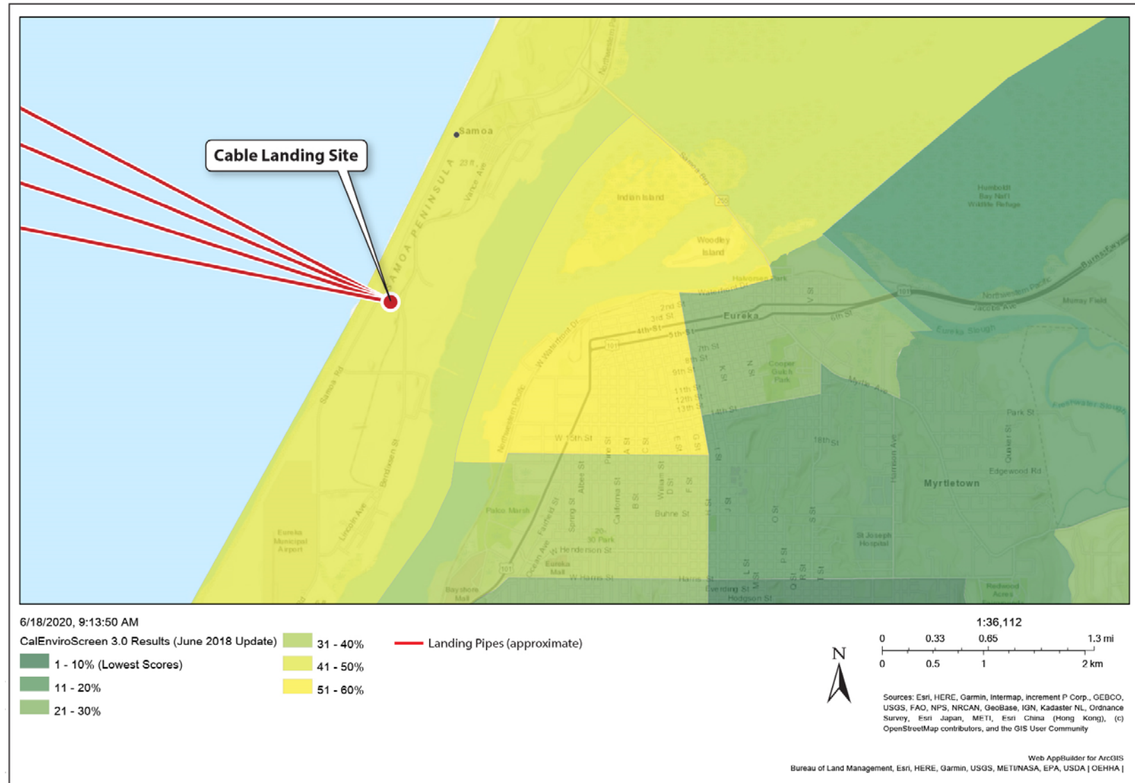
Figure 5-1. CalEnviroScreen Assessment
