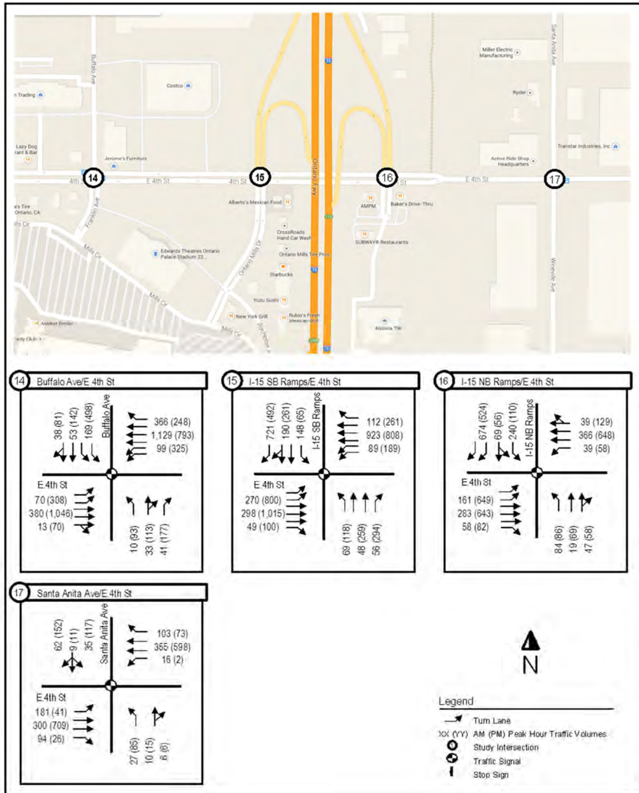
Exhibit 35: Existing (2014) Intersection Volumes (Continued)
