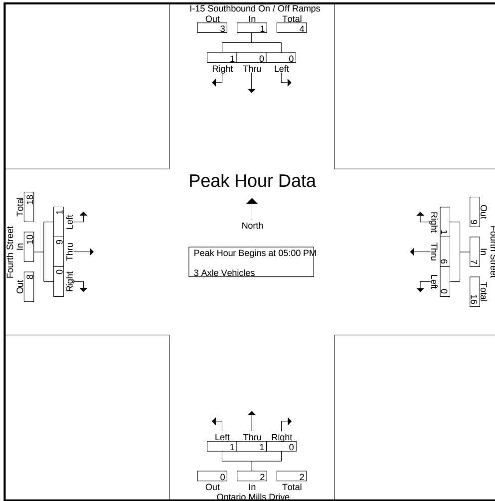
Peak Hour Analysis From 04:45 PM to 05:45 PM - Peak 1 of 1 Peak Hour for Each Approach Begins at:
