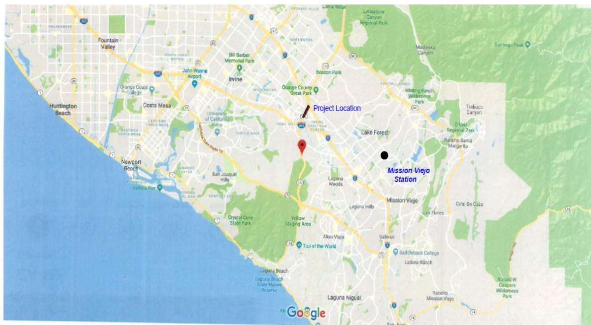
Figure 3-1. Map of the Air Quality Monitoring Station Located Near the Project Area
