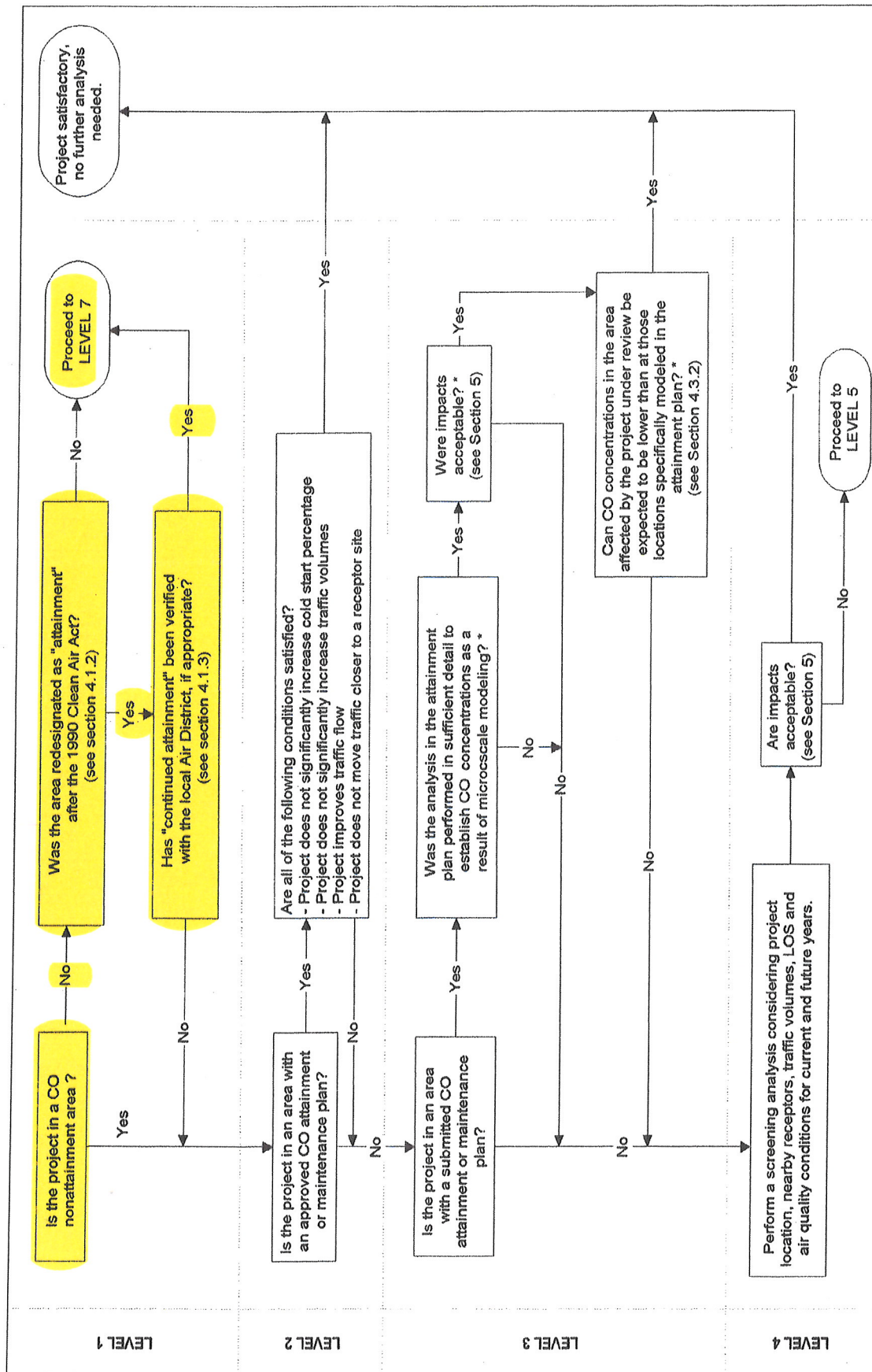
Figure 3. Local CO Analysis
