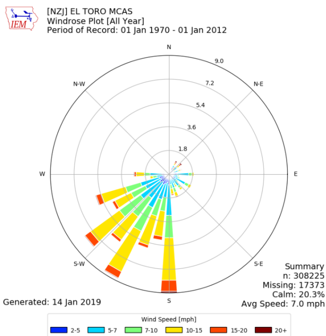
Figure 3-2. Predominant Wind Patterns at El Toro
