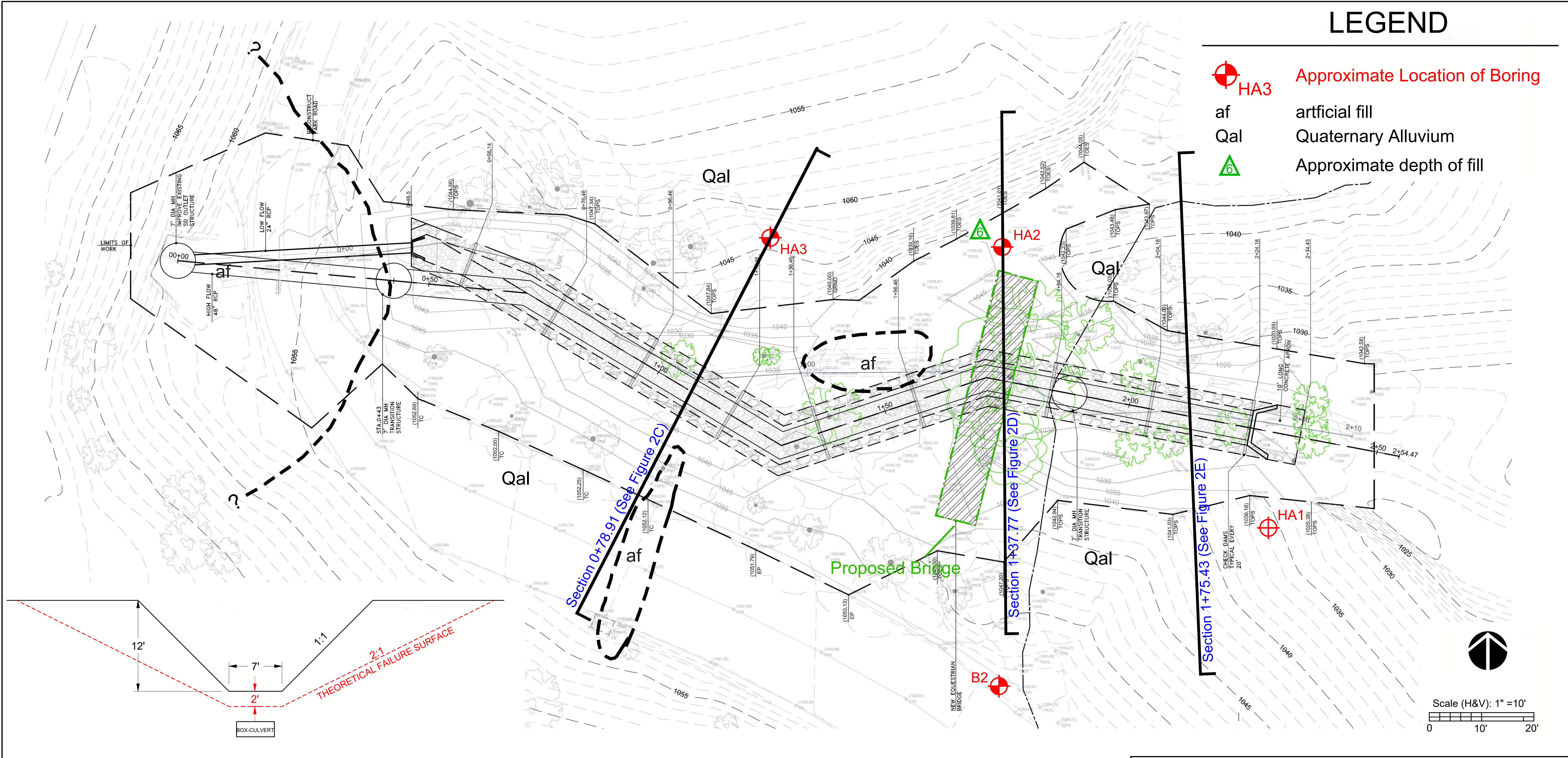
ILLUSTRATION OF PROPOSED CHANNEL CONFIGURATION FOR REFERENCE ONLY, NOT FOR CONSTRUCTION
