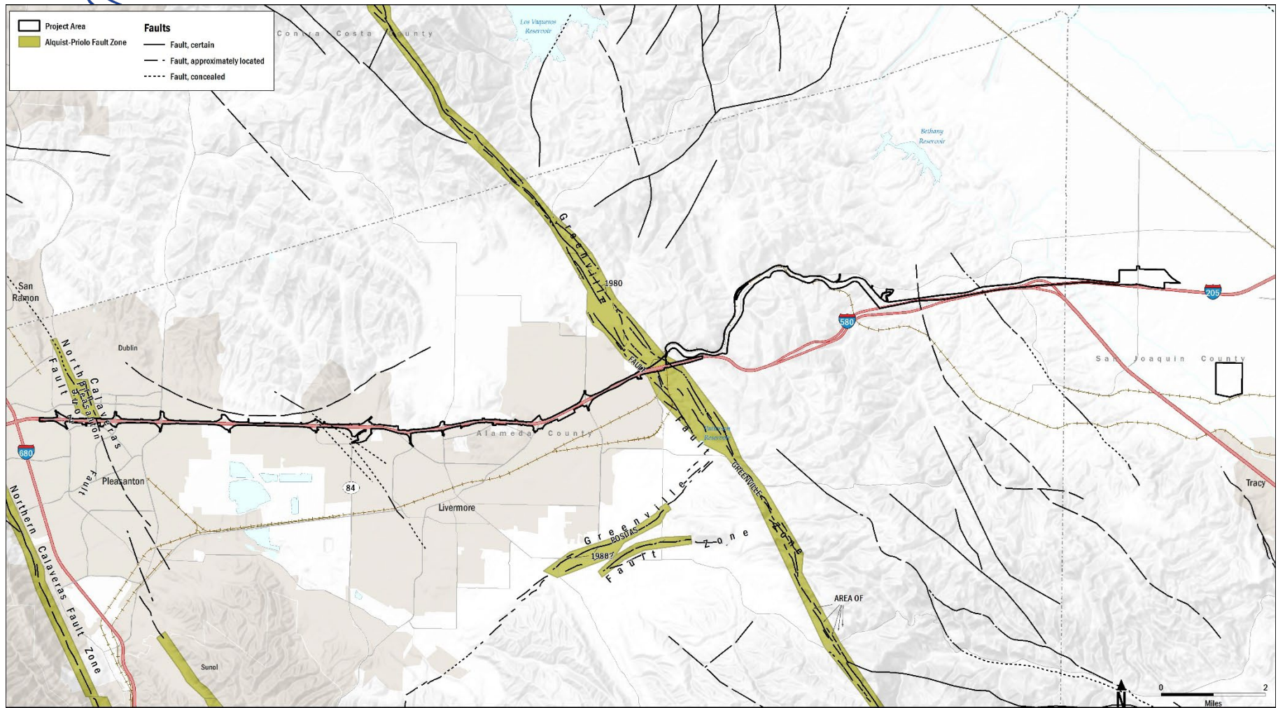
Figure A3.8-2: Alquist-Priolo Zones
