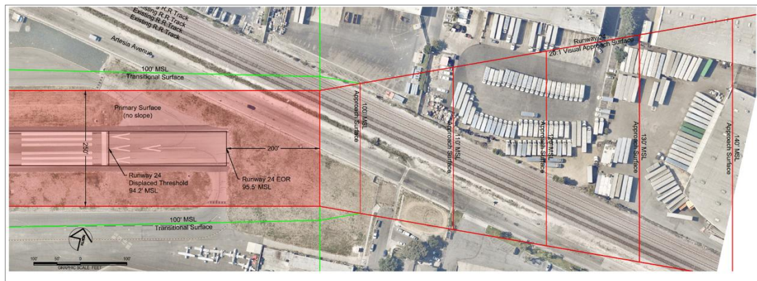
Figure 3.11-C-6 Fullerton Municipal Airport: Existing Part 77 Surfaces for Runway 6-24
